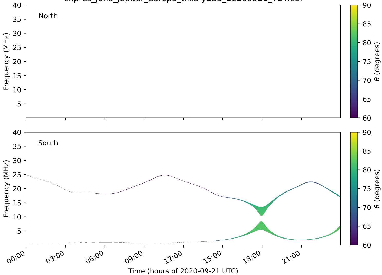
expres_juno_jupiter_europa_txka-y235_20200921_v14.cdf
