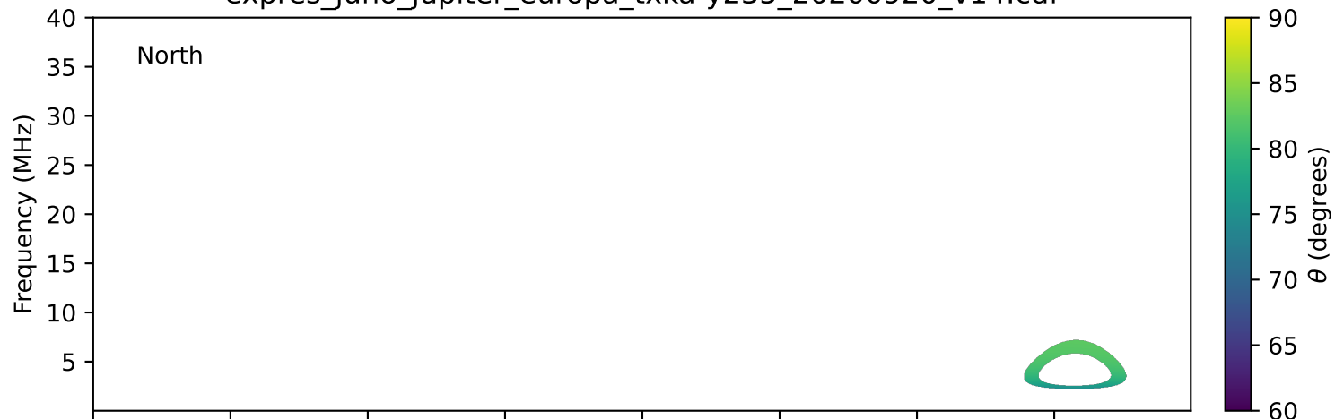
expres_juno_jupiter_europa_txka-y235_20200920_v14.cdf
