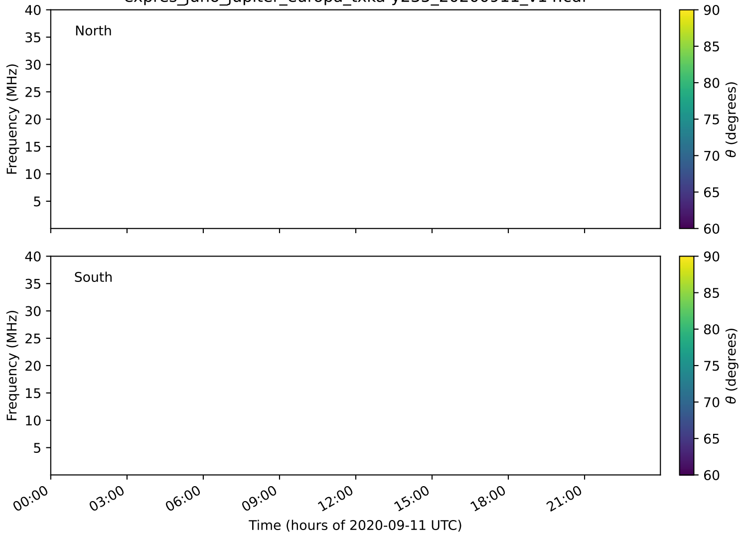
expres_juno_jupiter_europa_txka-y235_20200911_v14.cdf
