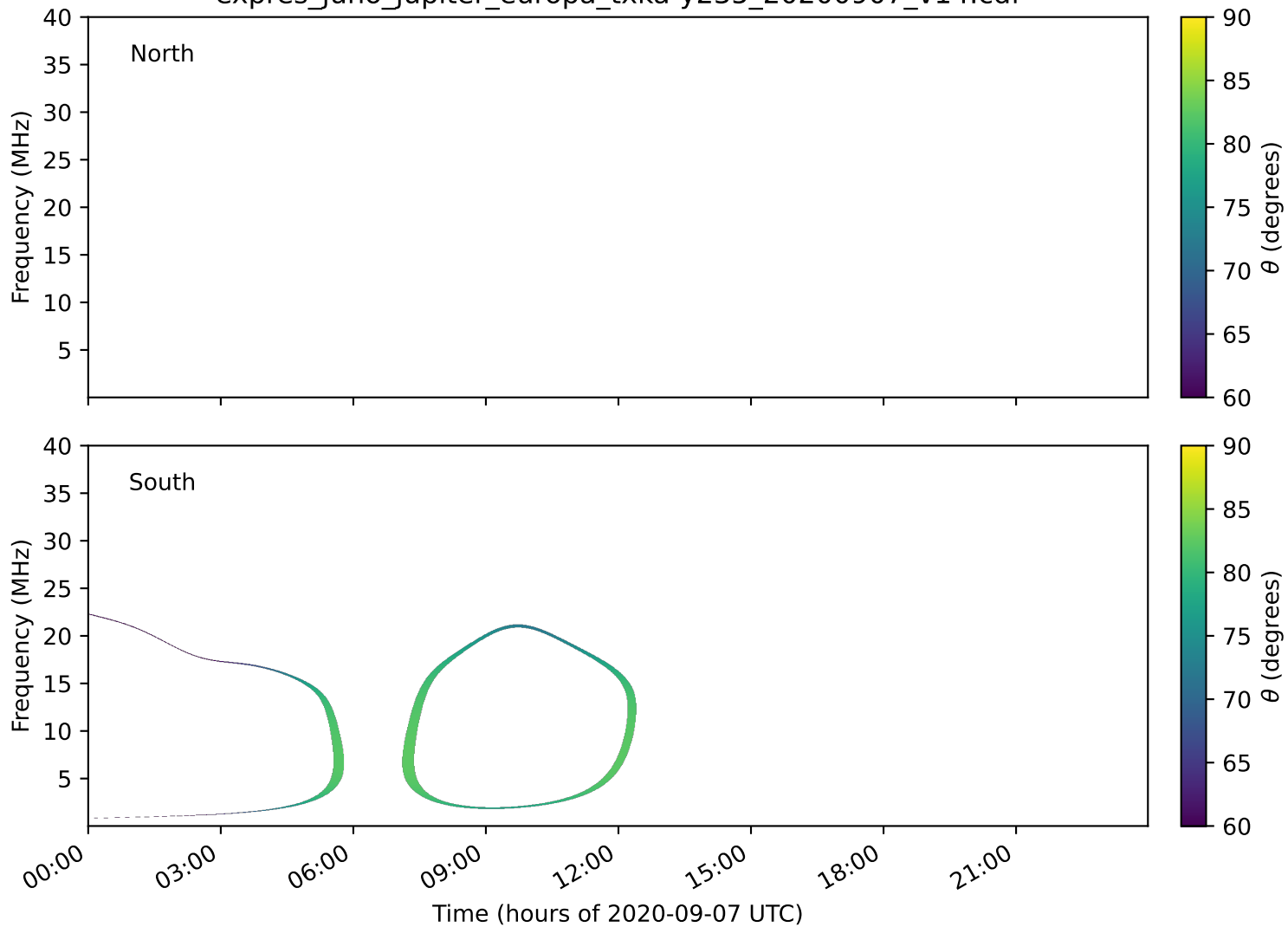
expres_juno_jupiter_europa_txka-y235_20200907_v14.cdf
