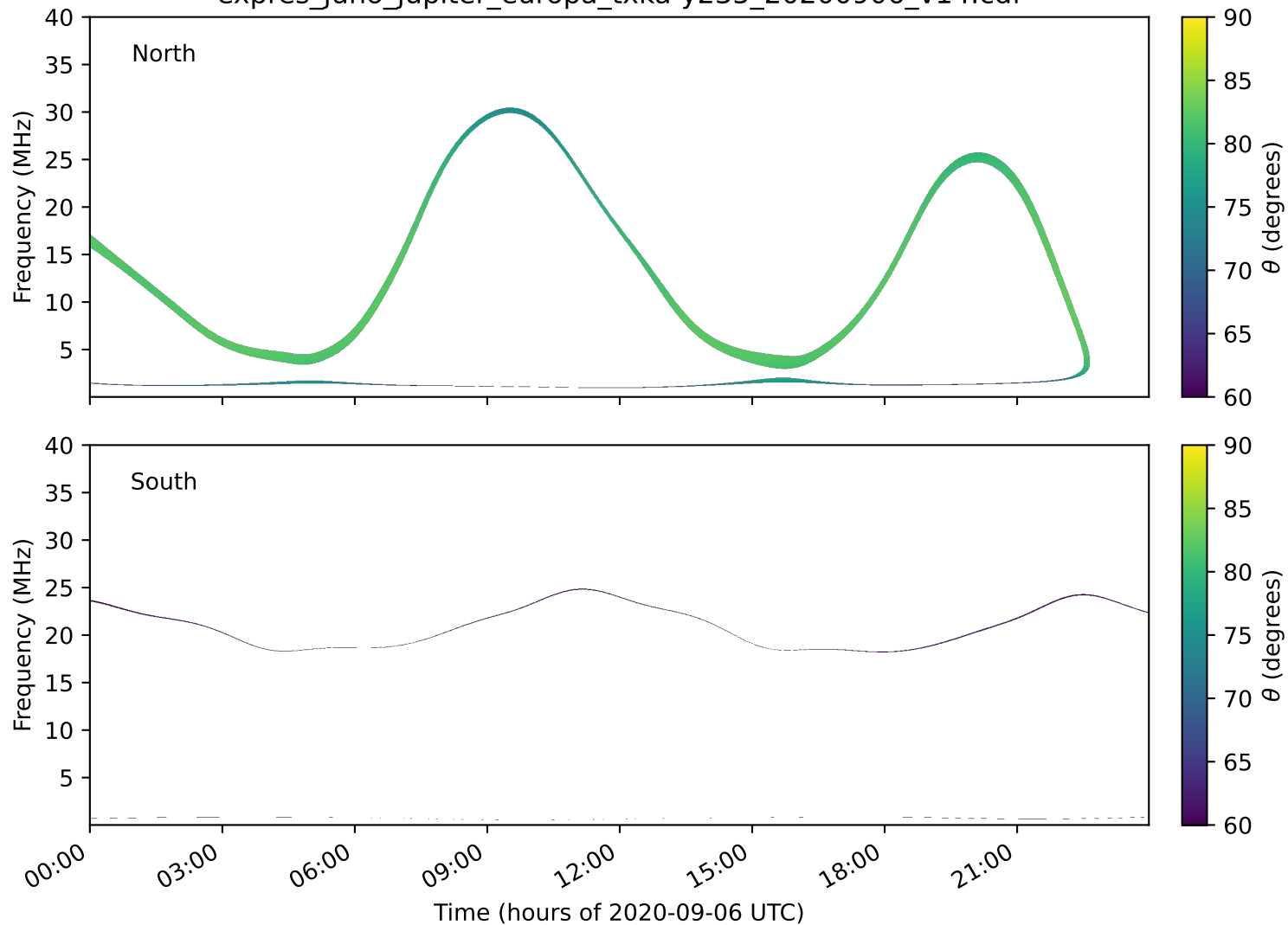
expres_juno_jupiter_europa_txka-y235_20200906_v14.cdf
