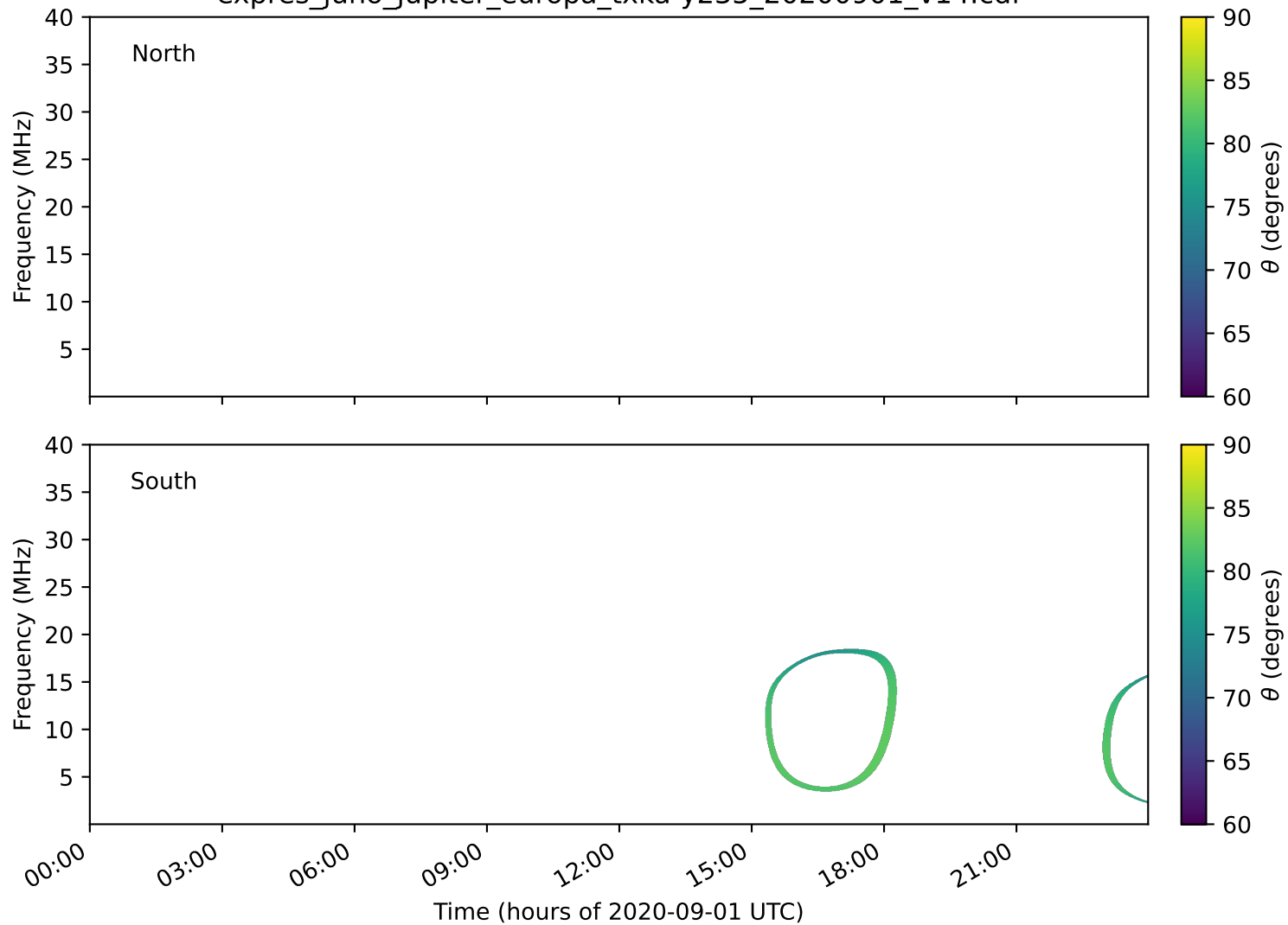
expres_juno_jupiter_europa_txka-y235_20200901_v14.cdf
