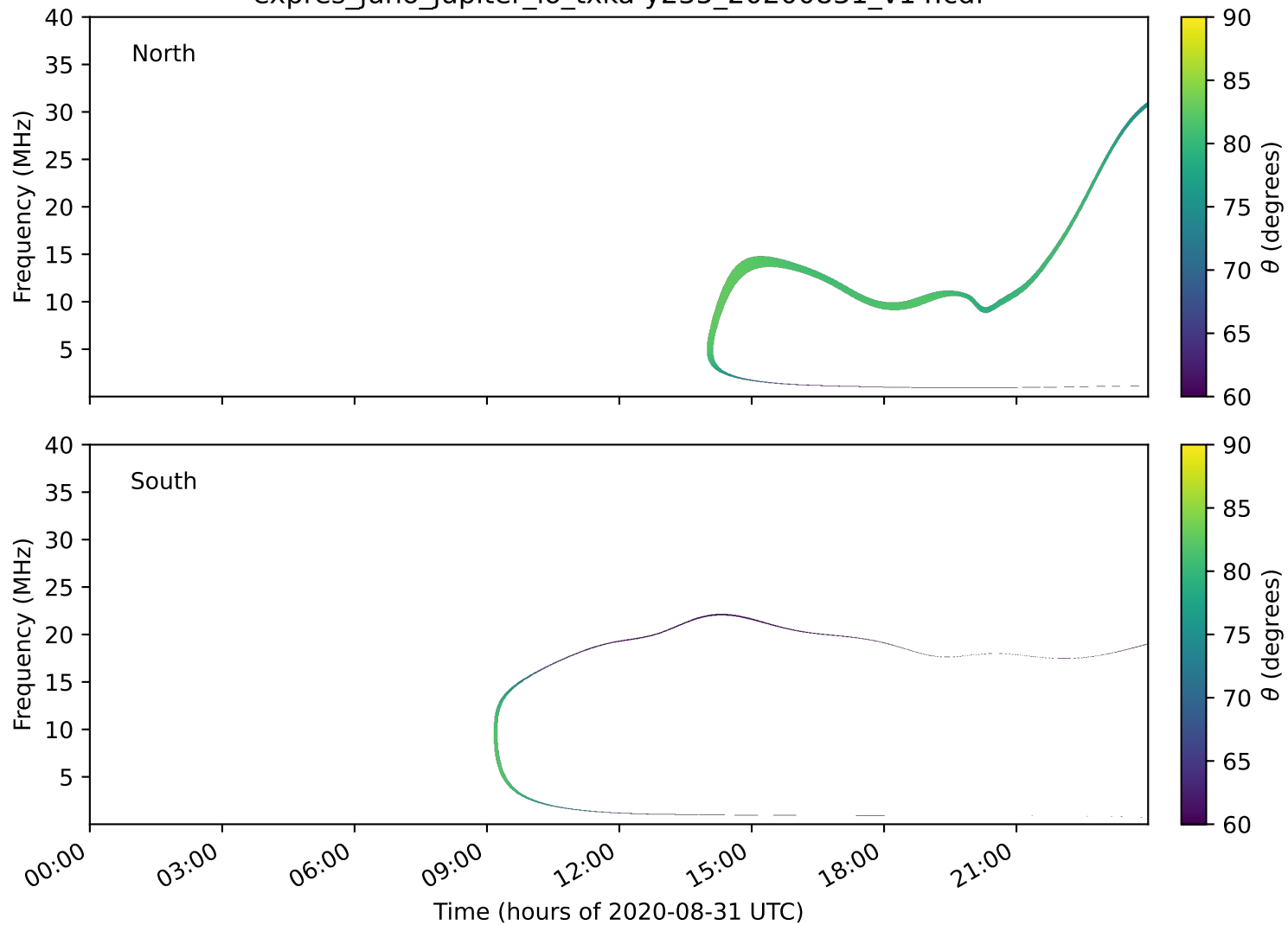
expres_juno_jupiter_io_txka-y235_20200831_v14.cdf
