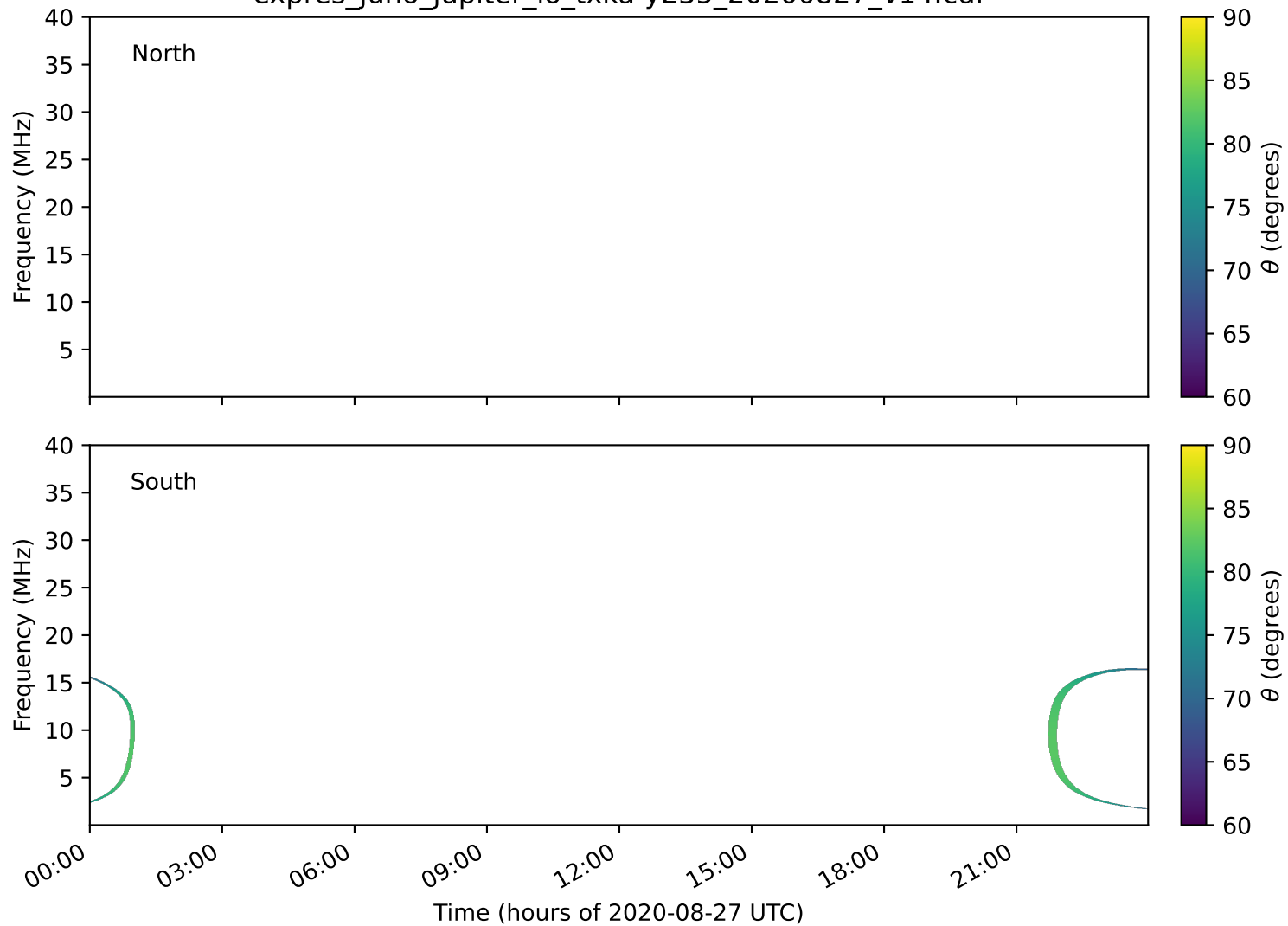
expres_juno_jupiter_io_txka-y235_20200827_v14.cdf
