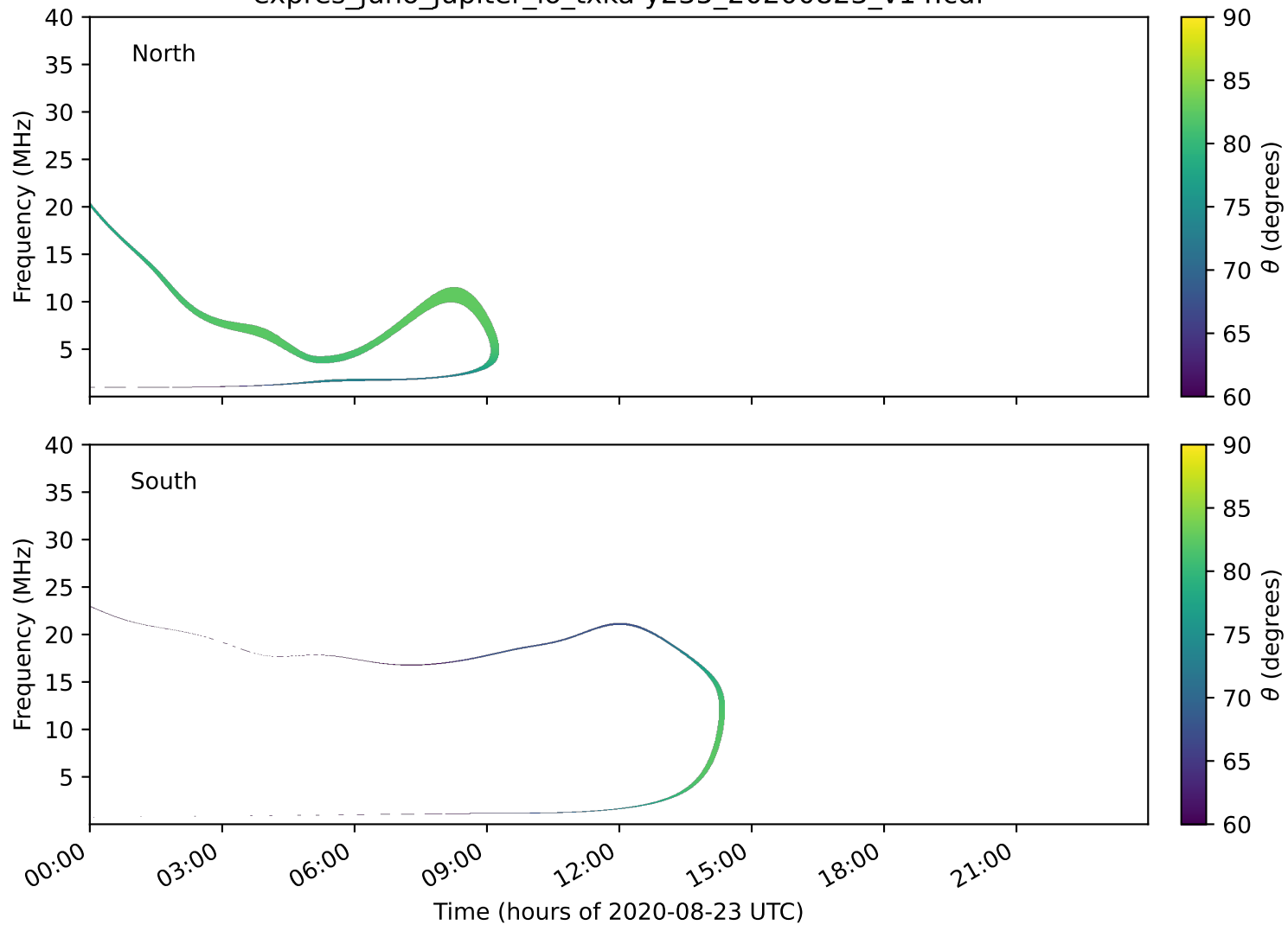
expres_juno_jupiter_io_txka-y235_20200823_v14.cdf
