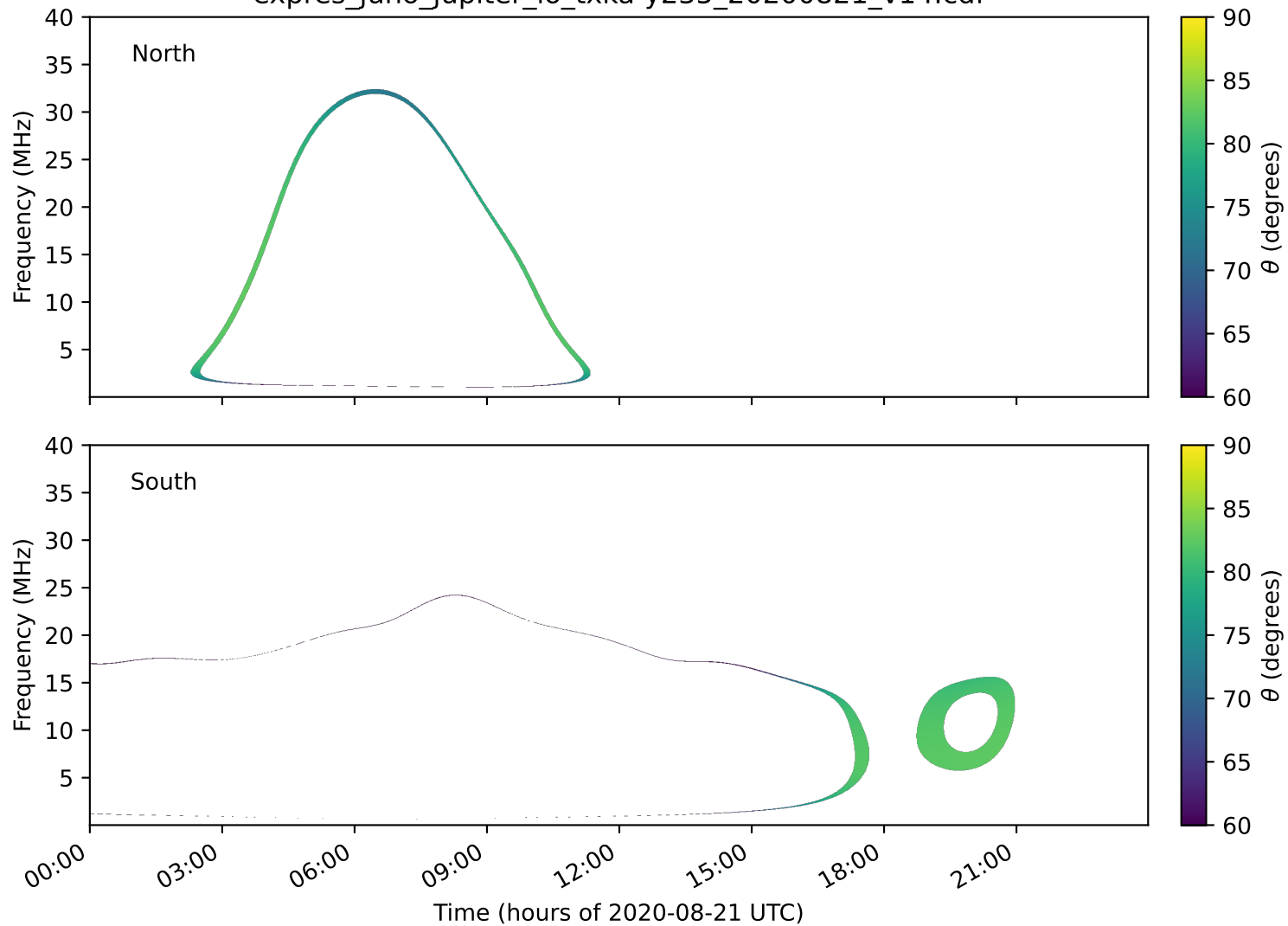
expres_juno_jupiter_io_txka-y235_20200821_v14.cdf
