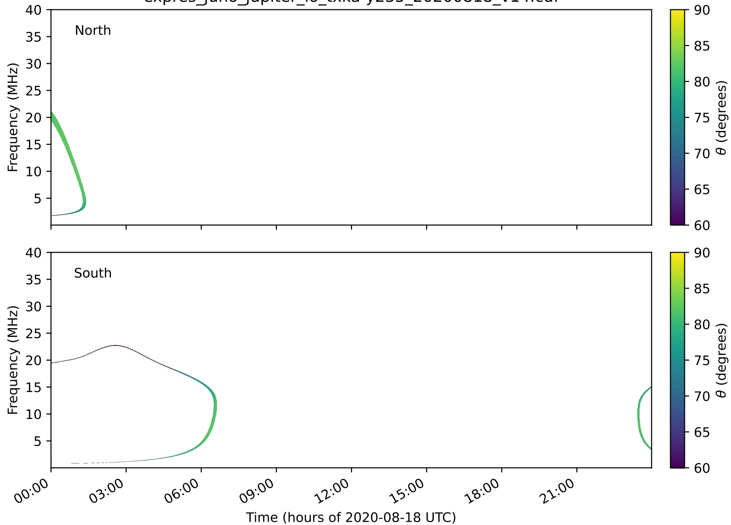
expres_juno_jupiter_io_txka-y235_20200818_v14.cdf
