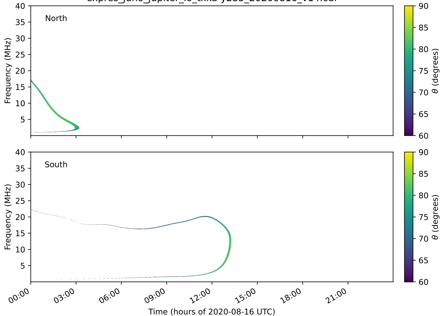
expres_juno_jupiter_io_txka-y235_20200816_v14.cdf
