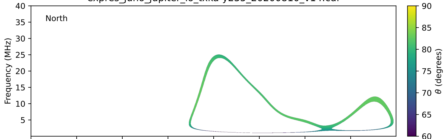
expres_juno_jupiter_io_txka-y235_20200810_v14.cdf
