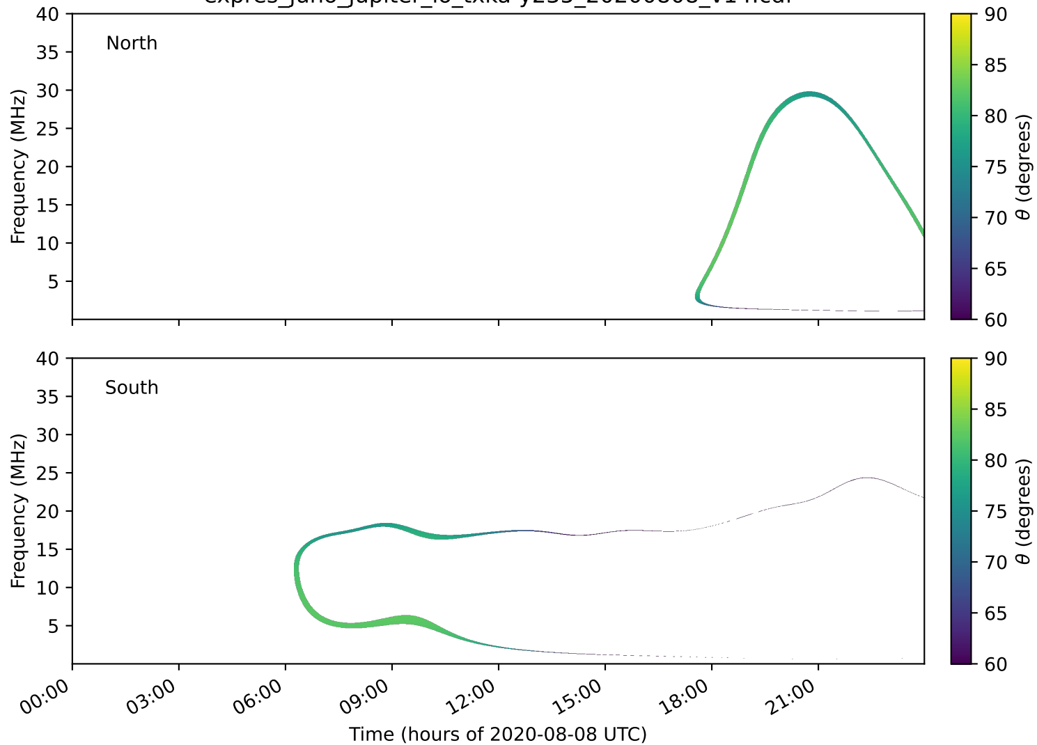
expres_juno_jupiter_io_txka-y235_20200808_v14.cdf
