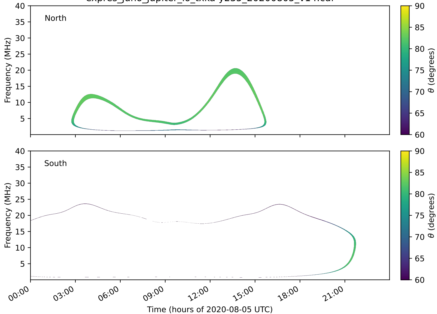
expres_juno_jupiter_io_txka-y235_20200805_v14.cdf
