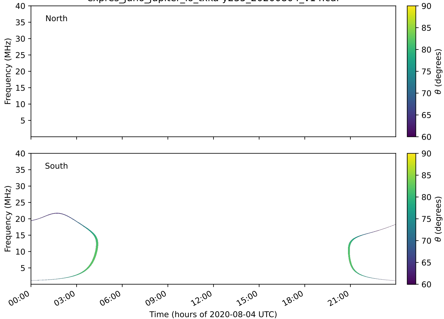
expres_juno_jupiter_io_txka-y235_20200804_v14.cdf
