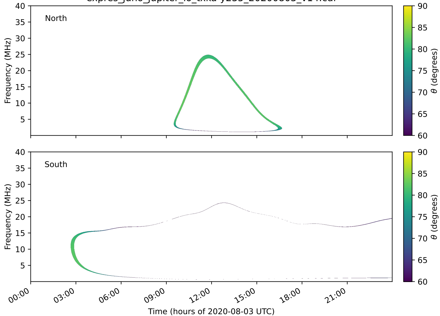
expres_juno_jupiter_io_txka-y235_20200803_v14.cdf
