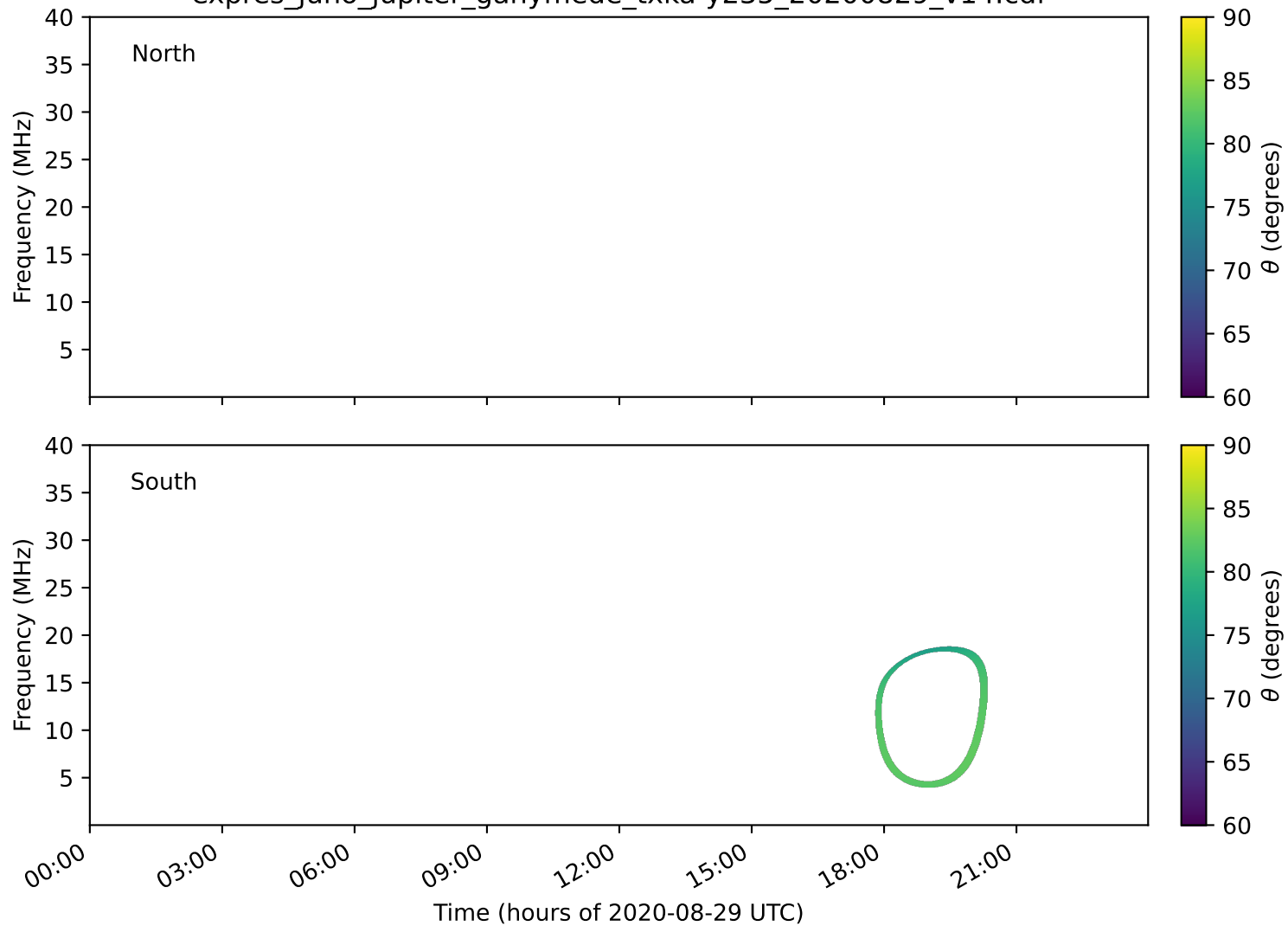
expres_juno_jupiter_ganymede_txka-y235_20200829_v14.cdf
