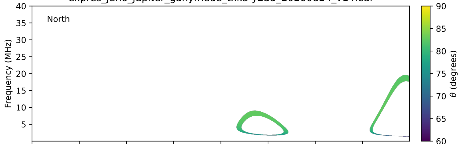
expres_juno_jupiter_ganymede_txka-y235_20200824_v14.cdf
