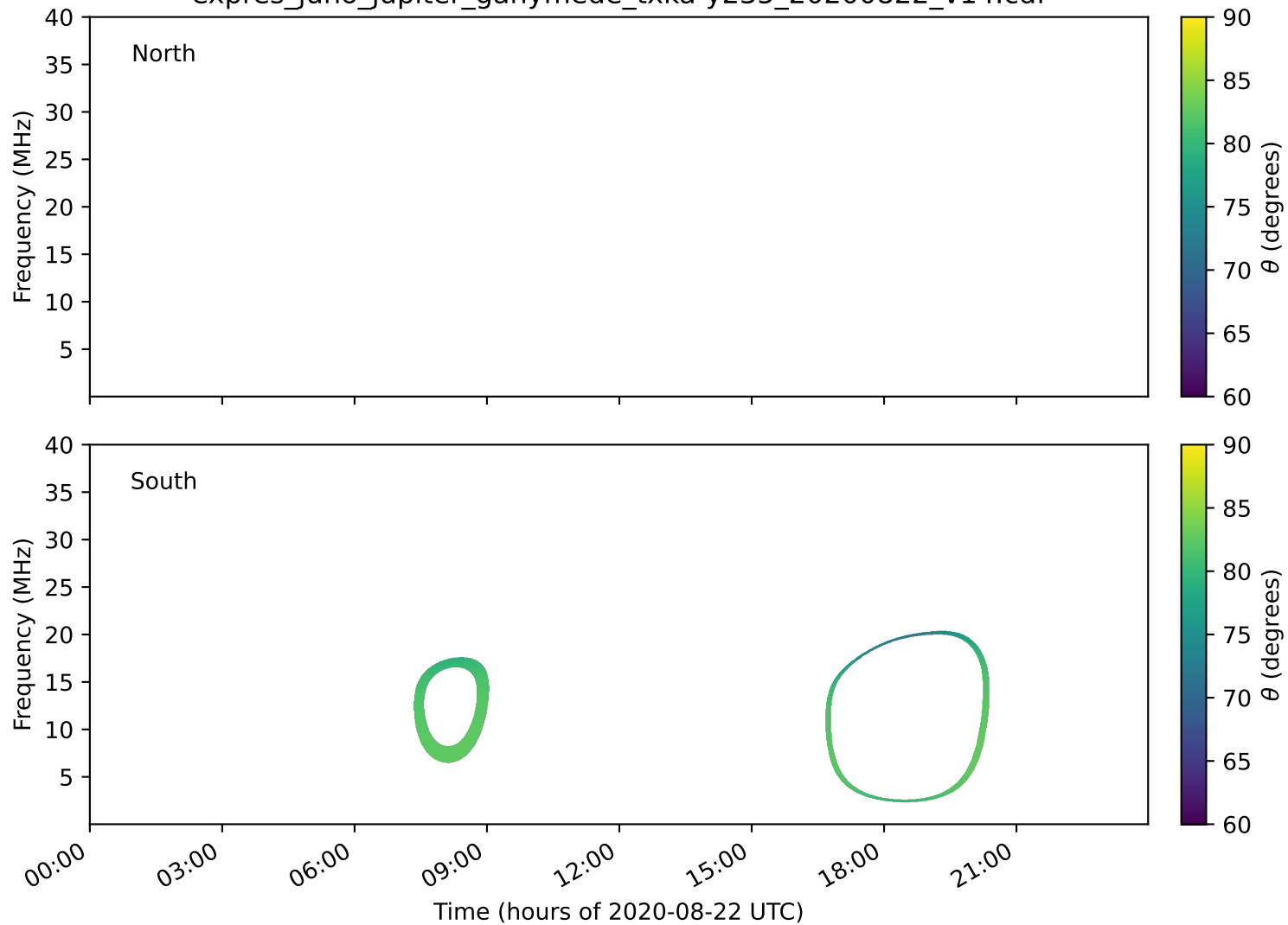
expres_juno_jupiter_ganymede_txka-y235_20200822_v14.cdf
