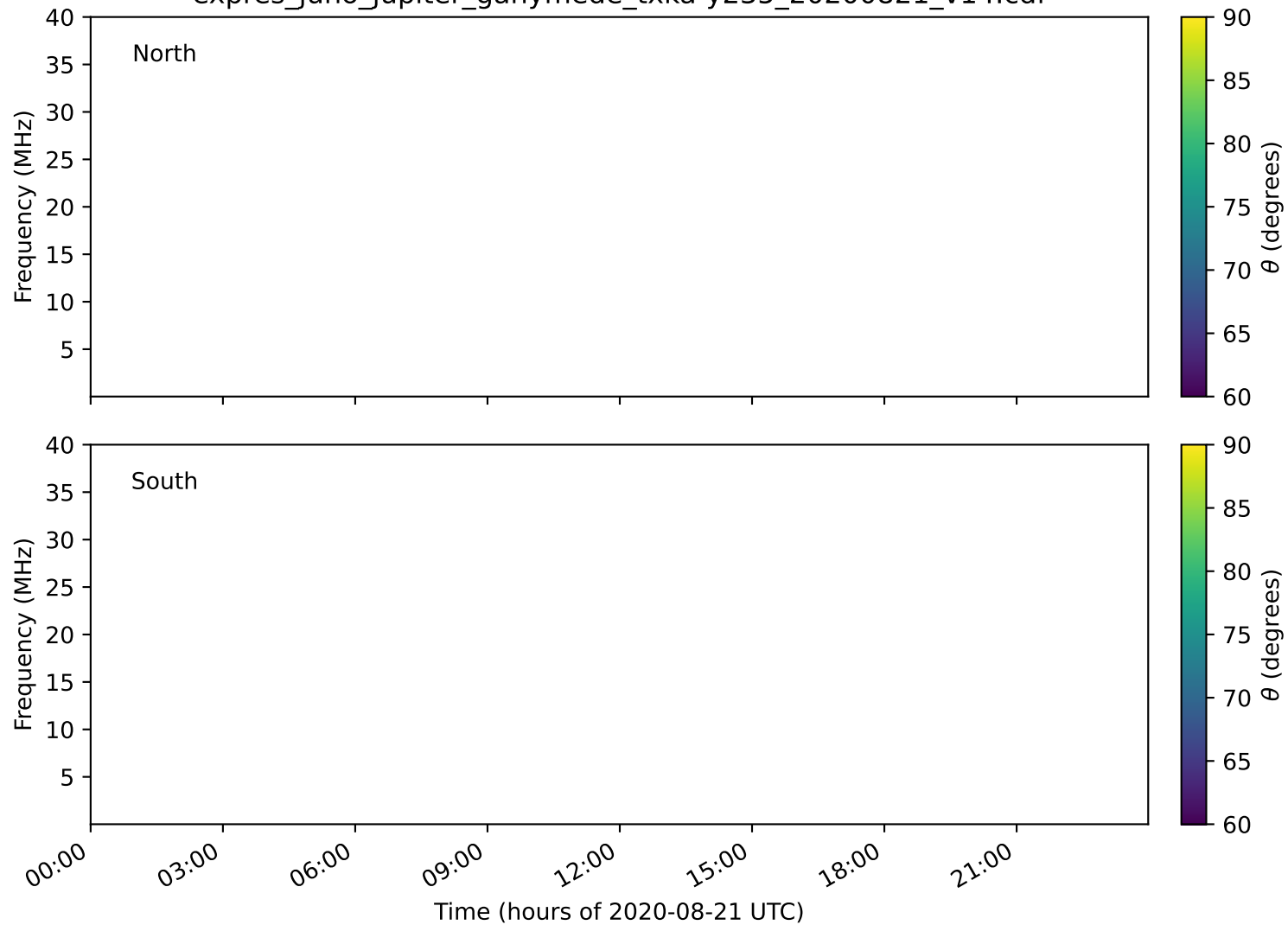
expres_juno_jupiter_ganymede_txka-y235_20200821_v14.cdf
