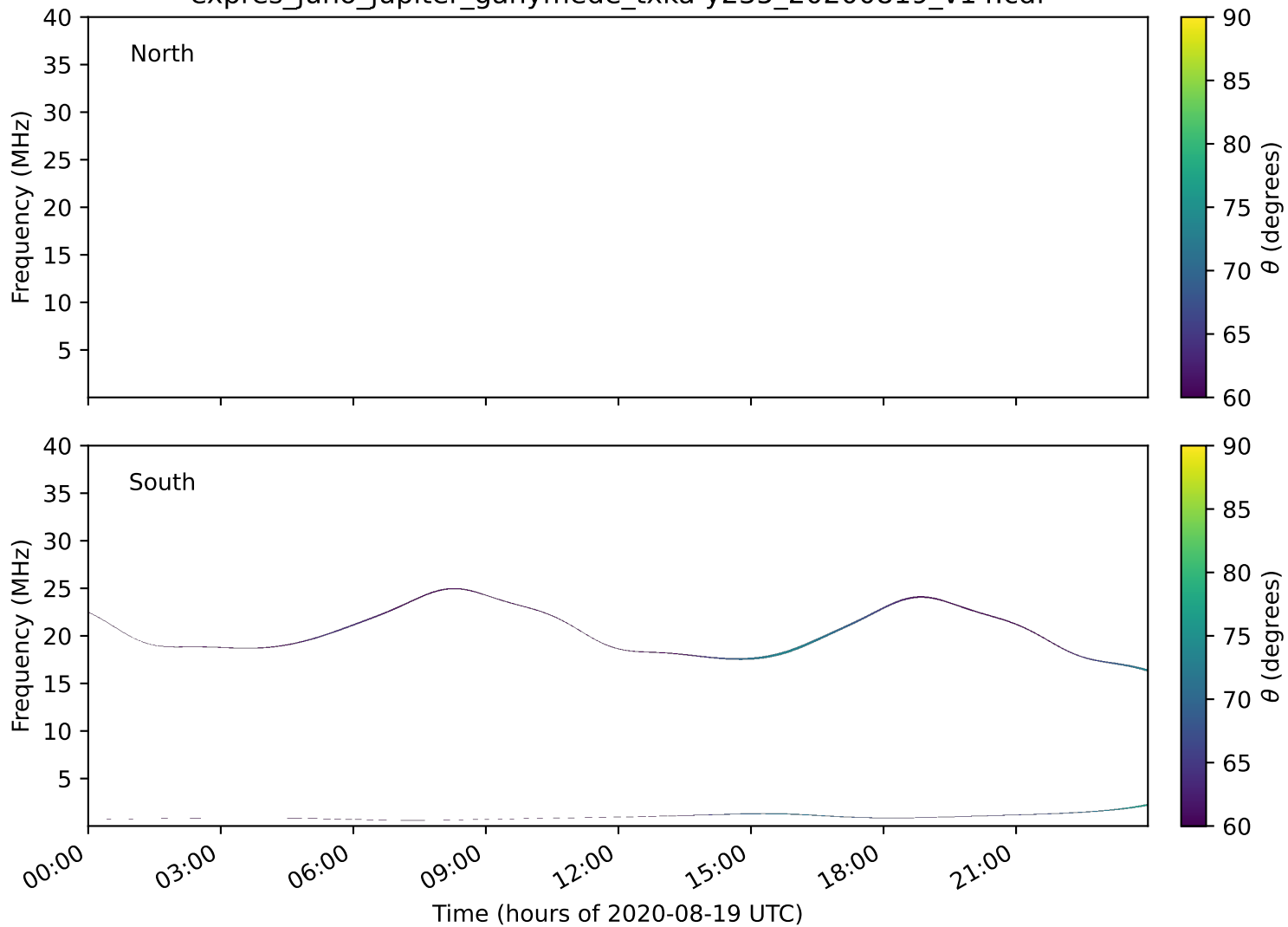
expres_juno_jupiter_ganymede_txka-y235_20200819_v14.cdf
