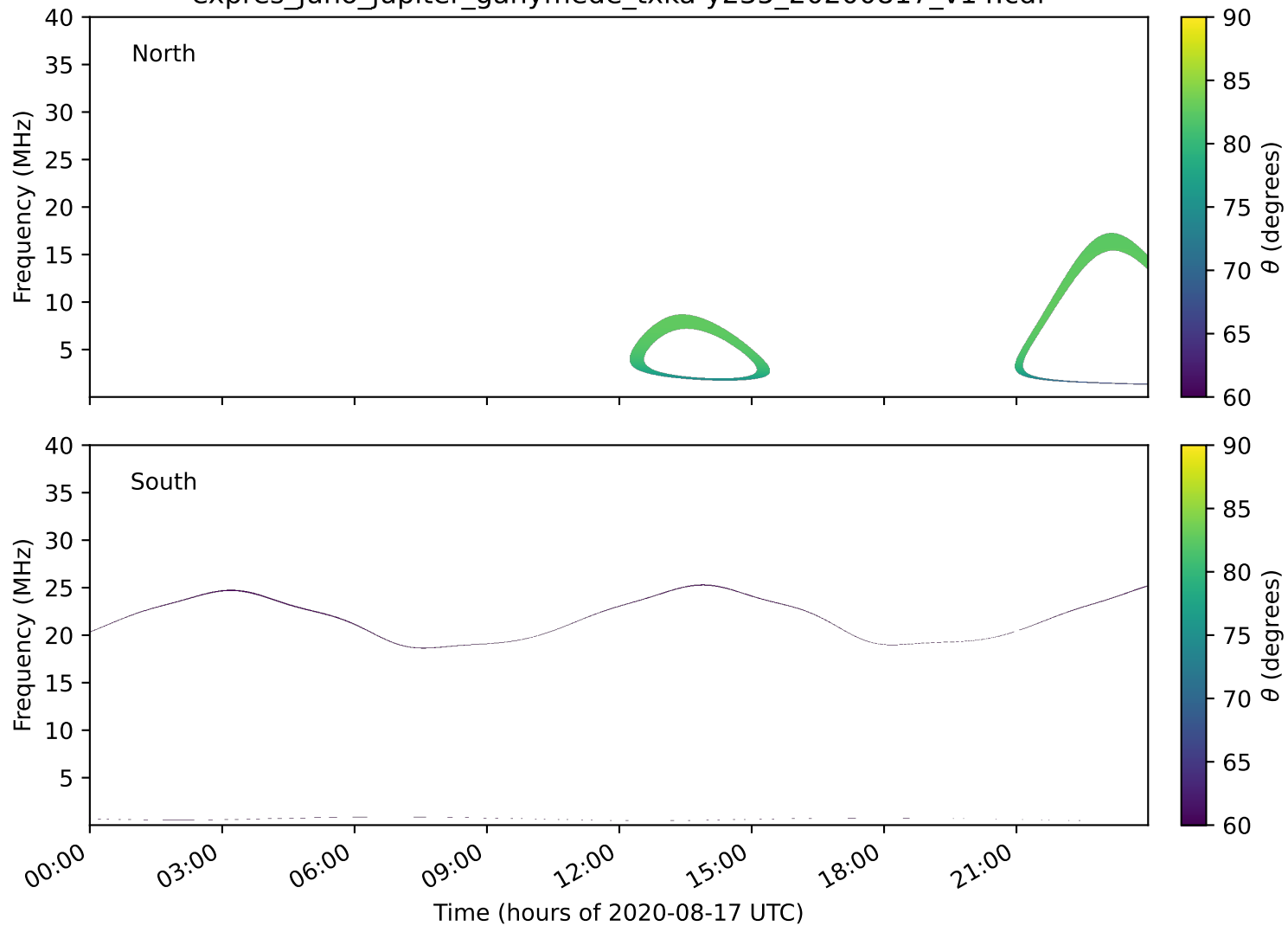
expres_juno_jupiter_ganymede_txka-y235_20200817_v14.cdf
