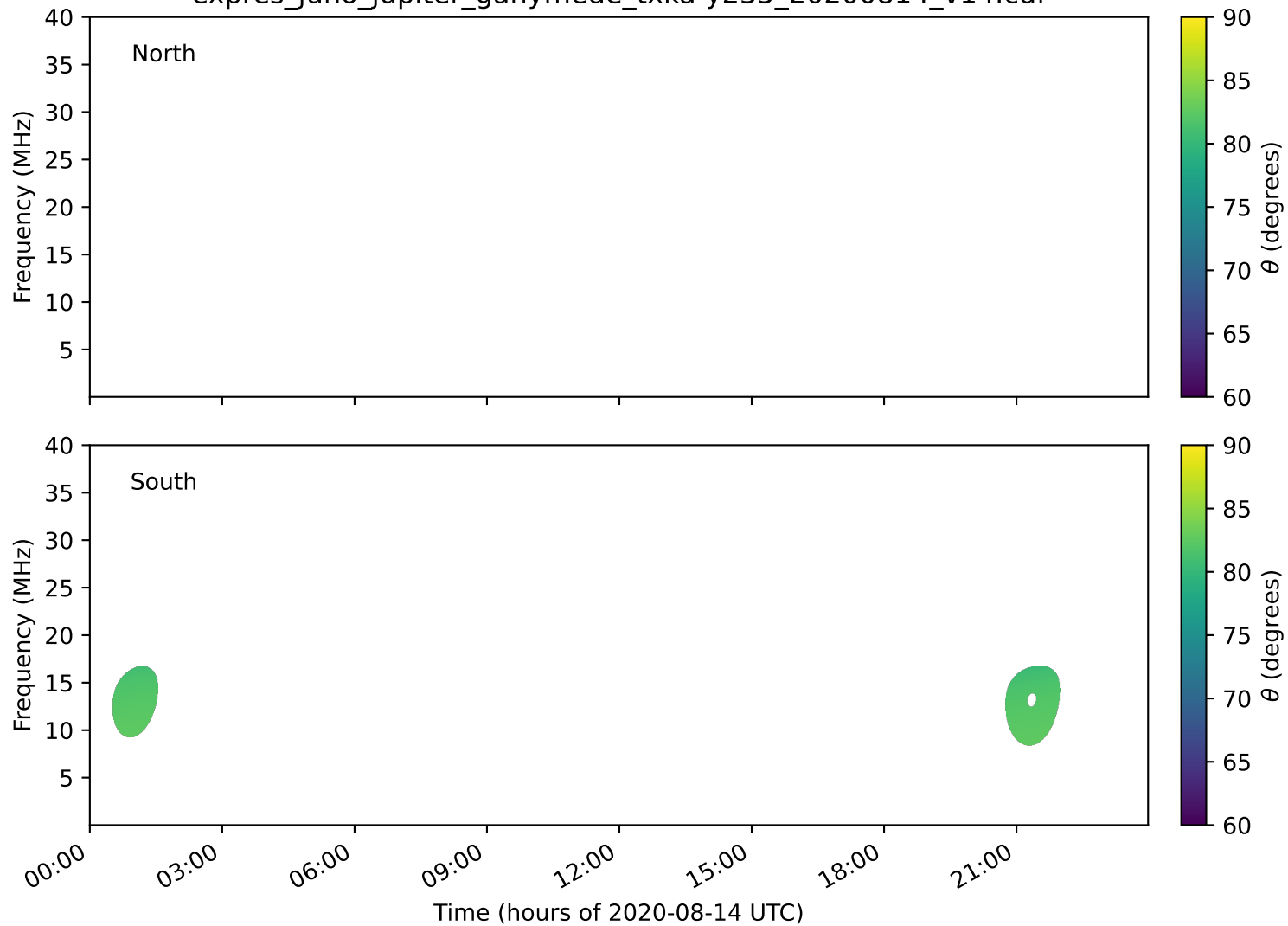
expres_juno_jupiter_ganymede_txka-y235_20200814_v14.cdf
