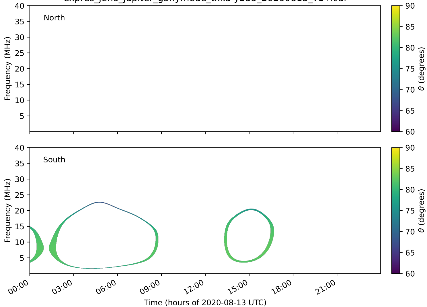
expres_juno_jupiter_ganymede_txka-y235_20200813_v14.cdf
