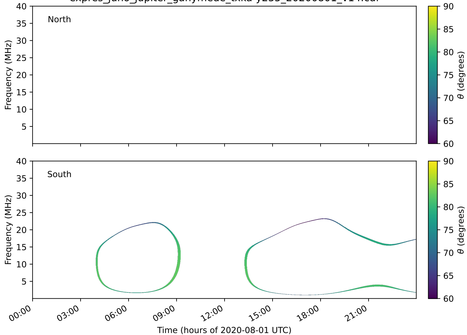
expres_juno_jupiter_ganymede_txka-y235_20200801_v14.cdf
