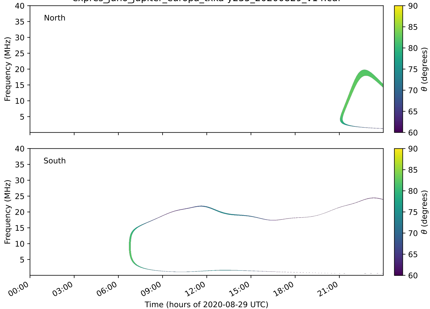
expres_juno_jupiter_europa_txka-y235_20200829_v14.cdf
