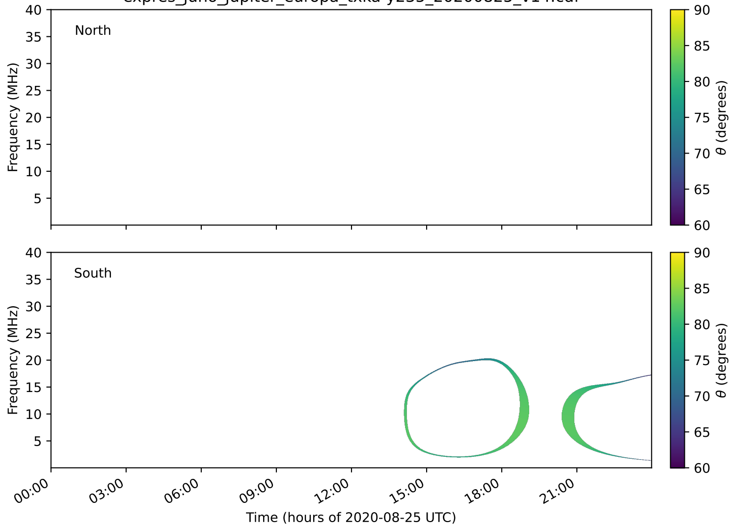
expres_juno_jupiter_europa_txka-y235_20200825_v14.cdf
