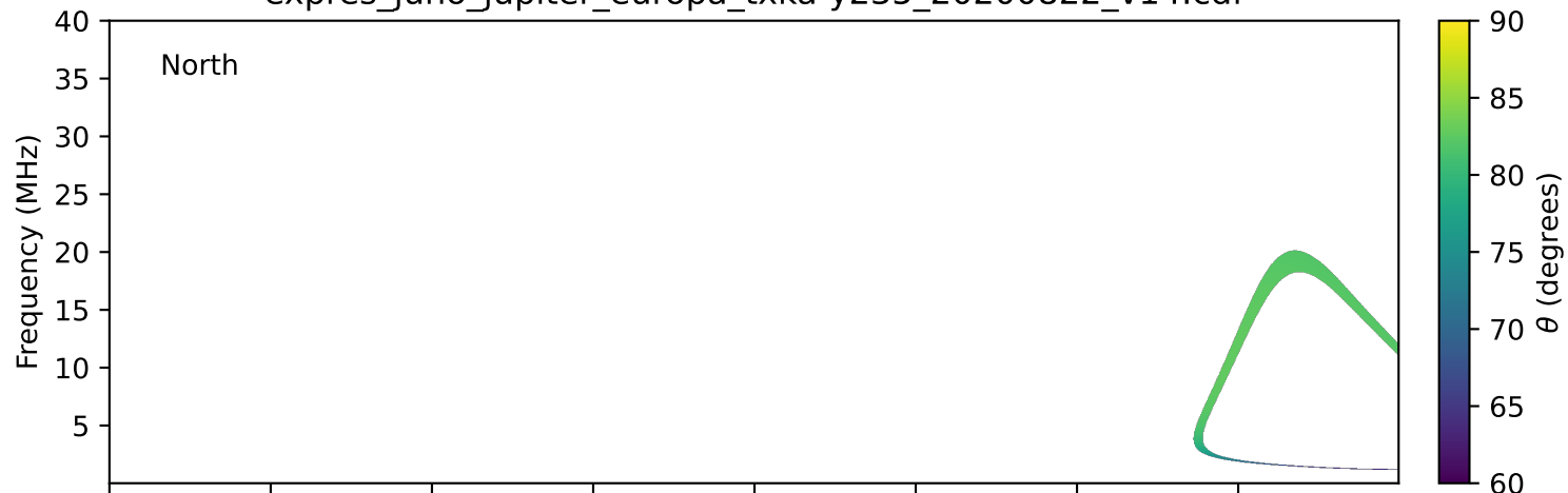
expres_juno_jupiter_europa_txka-y235_20200822_v14.cdf
