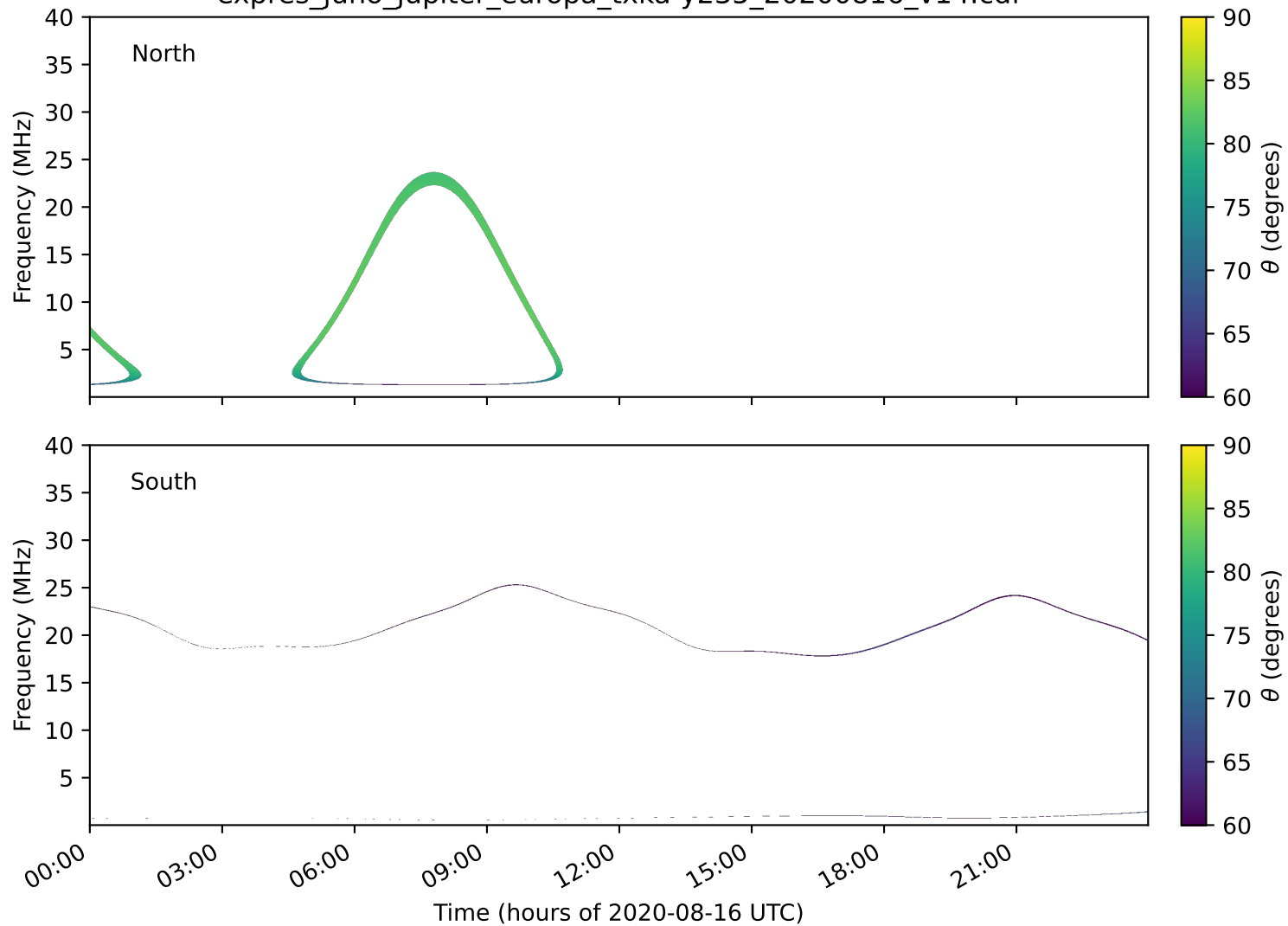
expres_juno_jupiter_europa_txka-y235_20200816_v14.cdf
