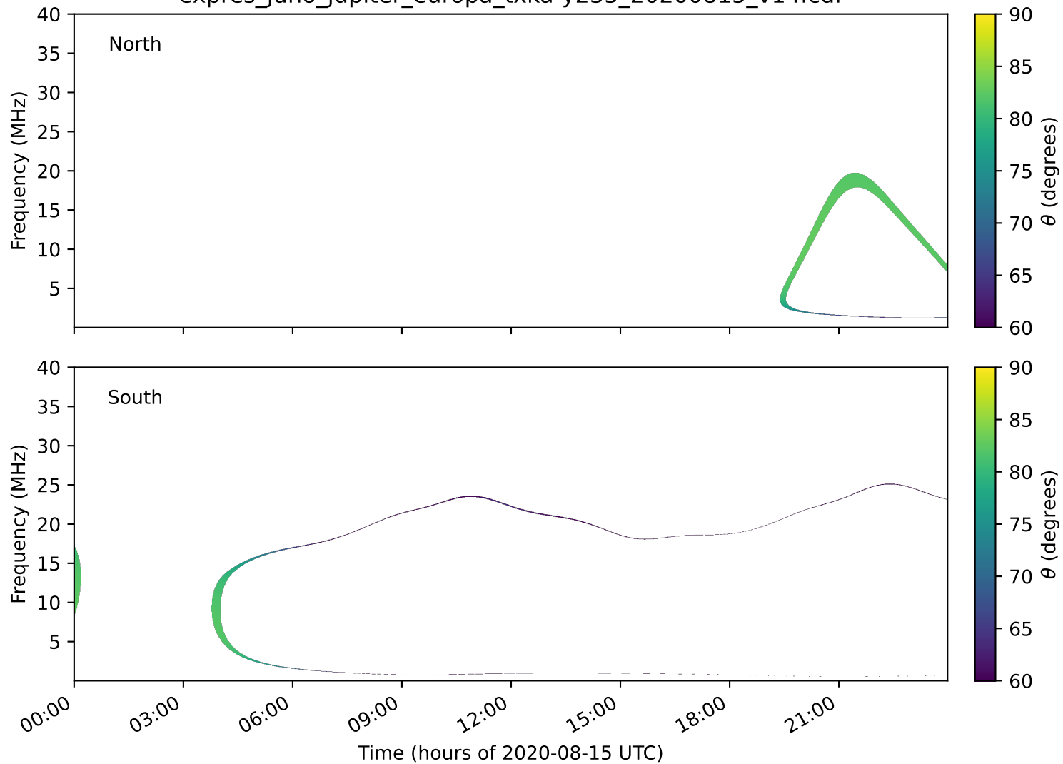
expres_juno_jupiter_europa_txka-y235_20200815_v14.cdf
