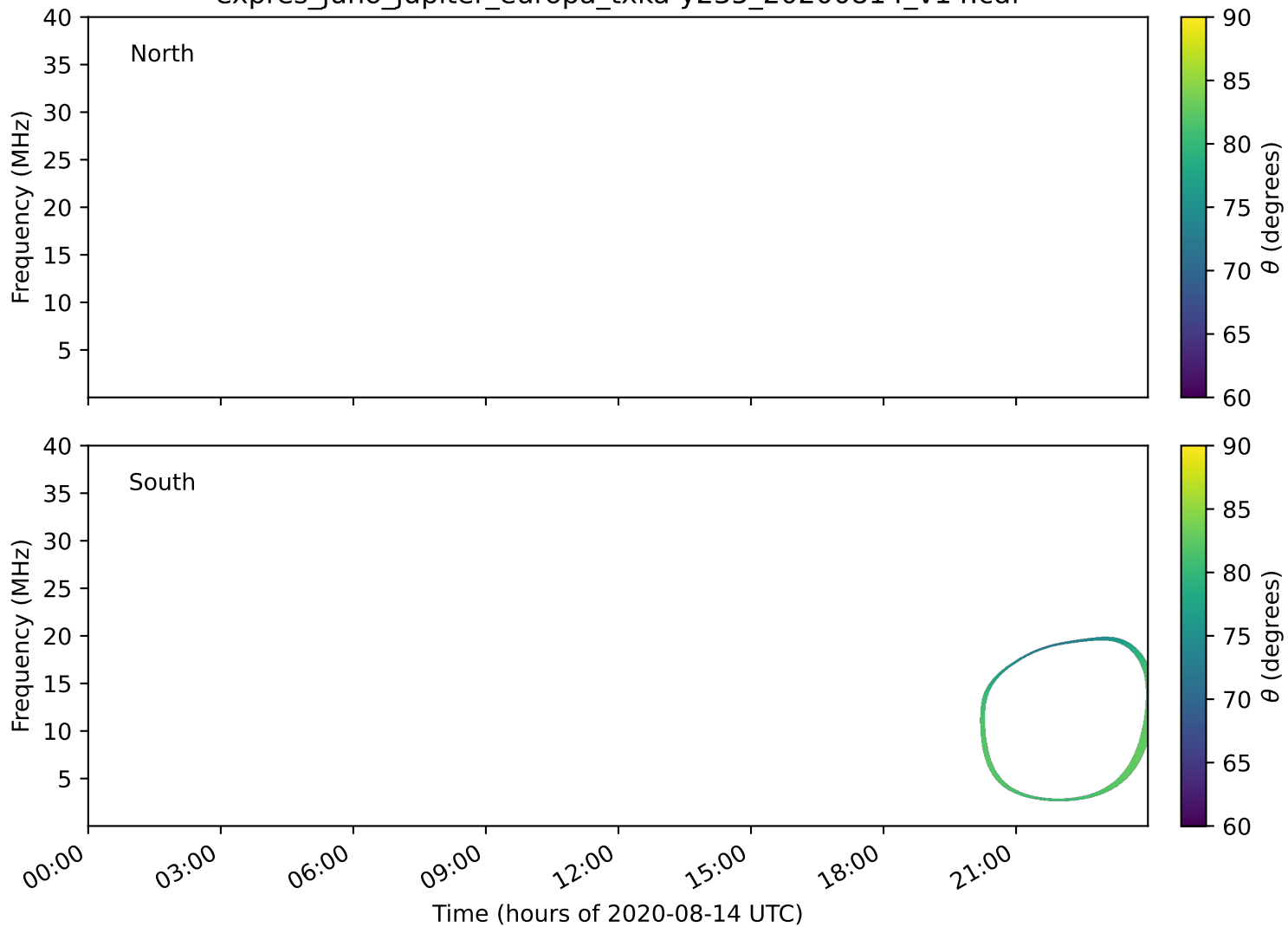
expres_juno_jupiter_europa_txka-y235_20200814_v14.cdf
