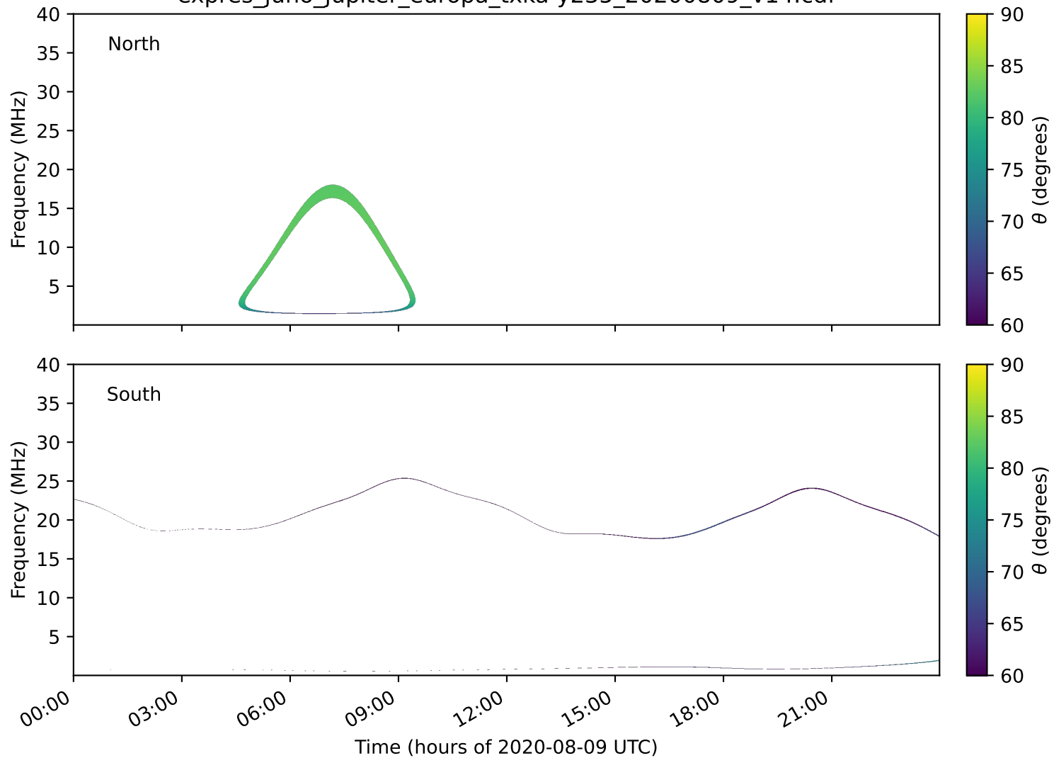
expres_juno_jupiter_europa_txka-y235_20200809_v14.cdf
