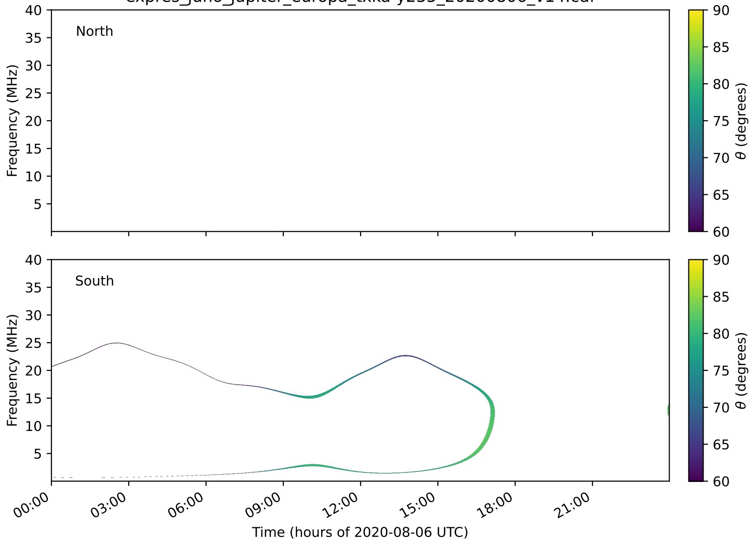
expres_juno_jupiter_europa_txka-y235_20200806_v14.cdf
