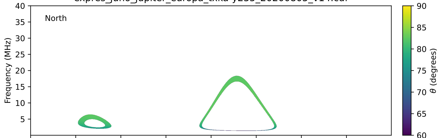
expres_juno_jupiter_europa_txka-y235_20200805_v14.cdf
