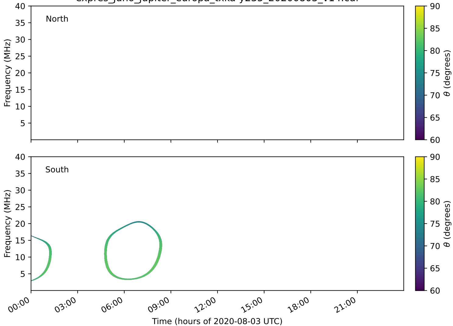
expres_juno_jupiter_europa_txka-y235_20200803_v14.cdf
