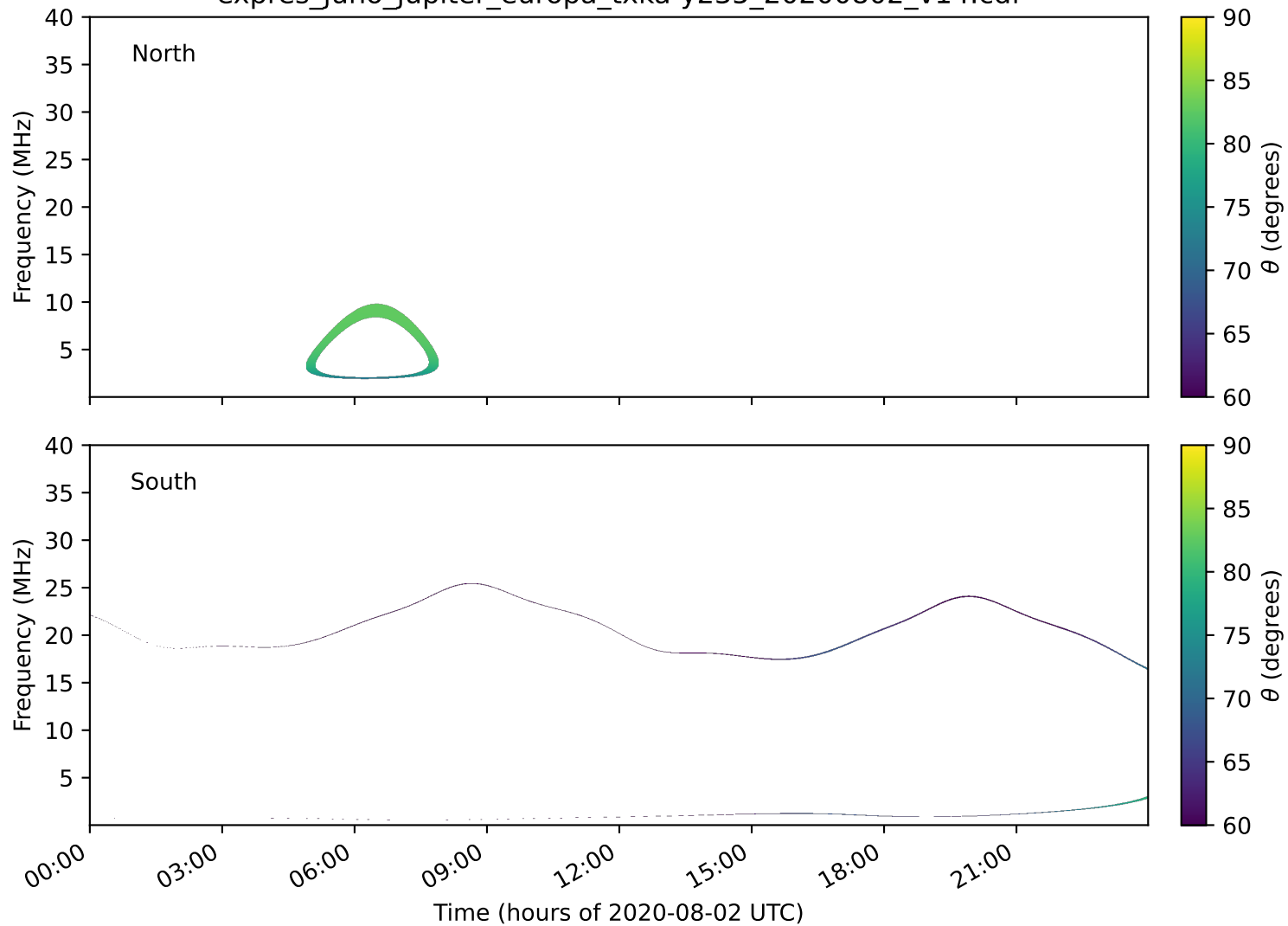
expres_juno_jupiter_europa_txka-y235_20200802_v14.cdf
