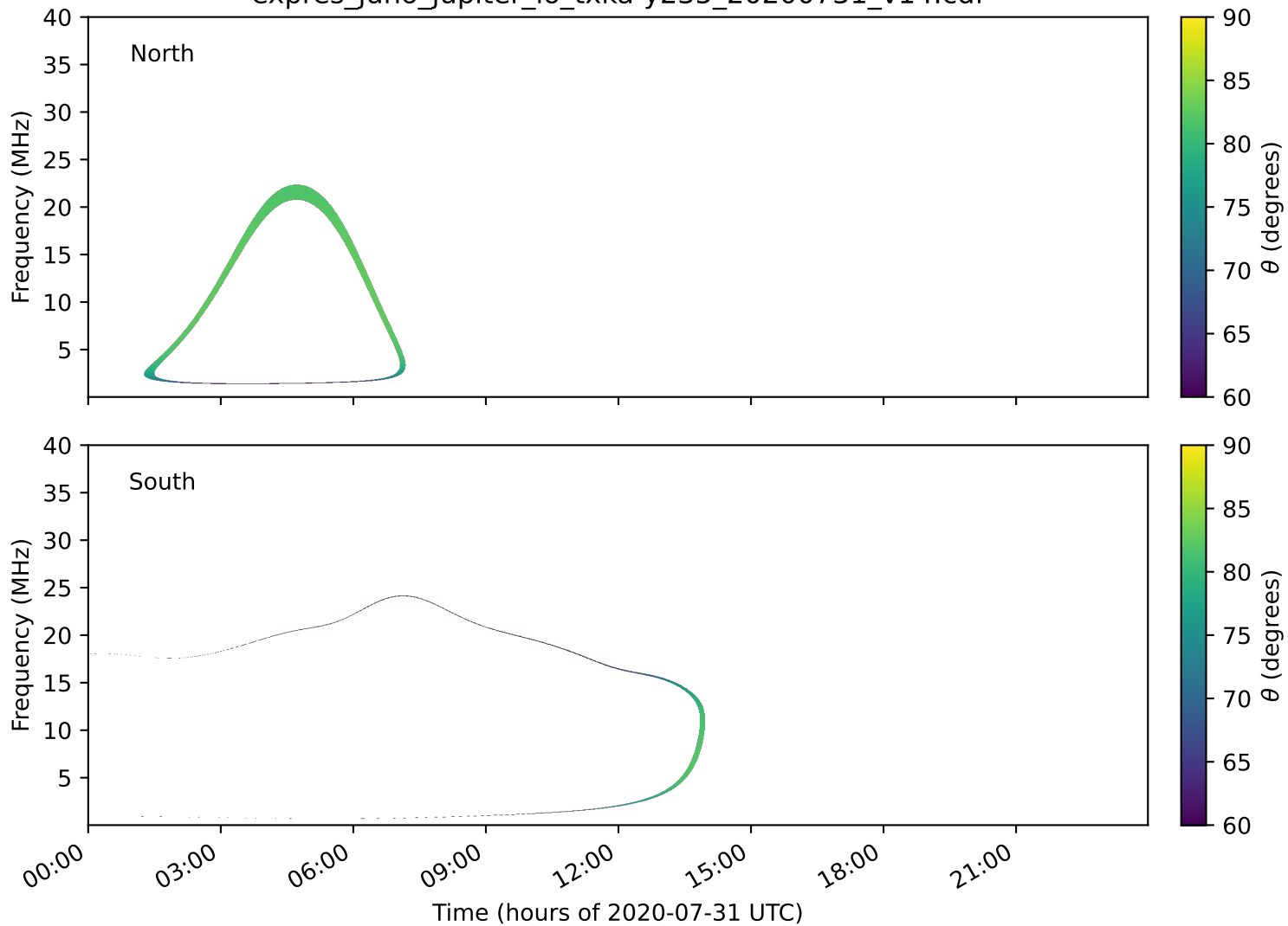
expres_juno_jupiter_io_txka-y235_20200731_v14.cdf
