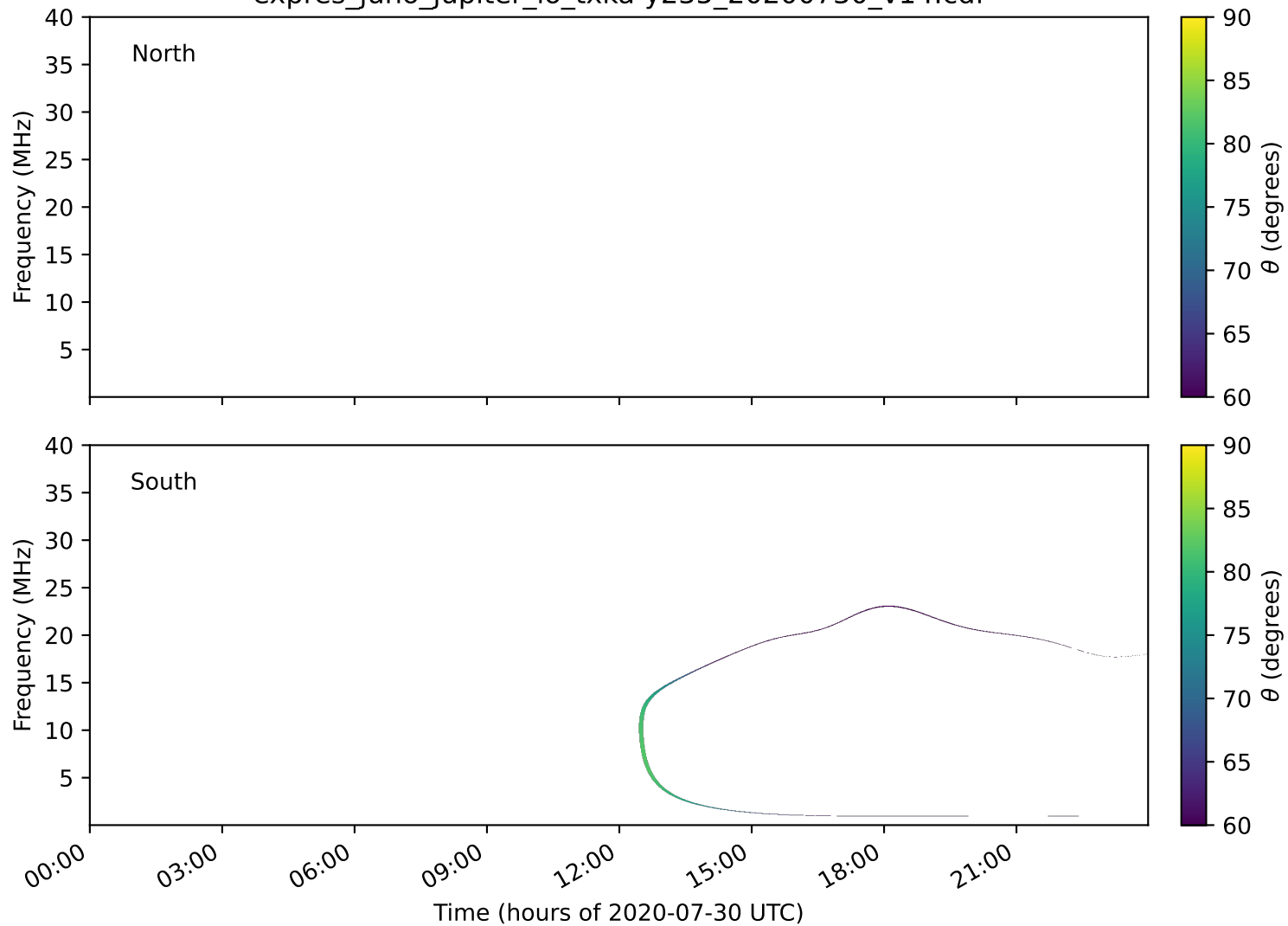
expres_juno_jupiter_io_txka-y235_20200730_v14.cdf
