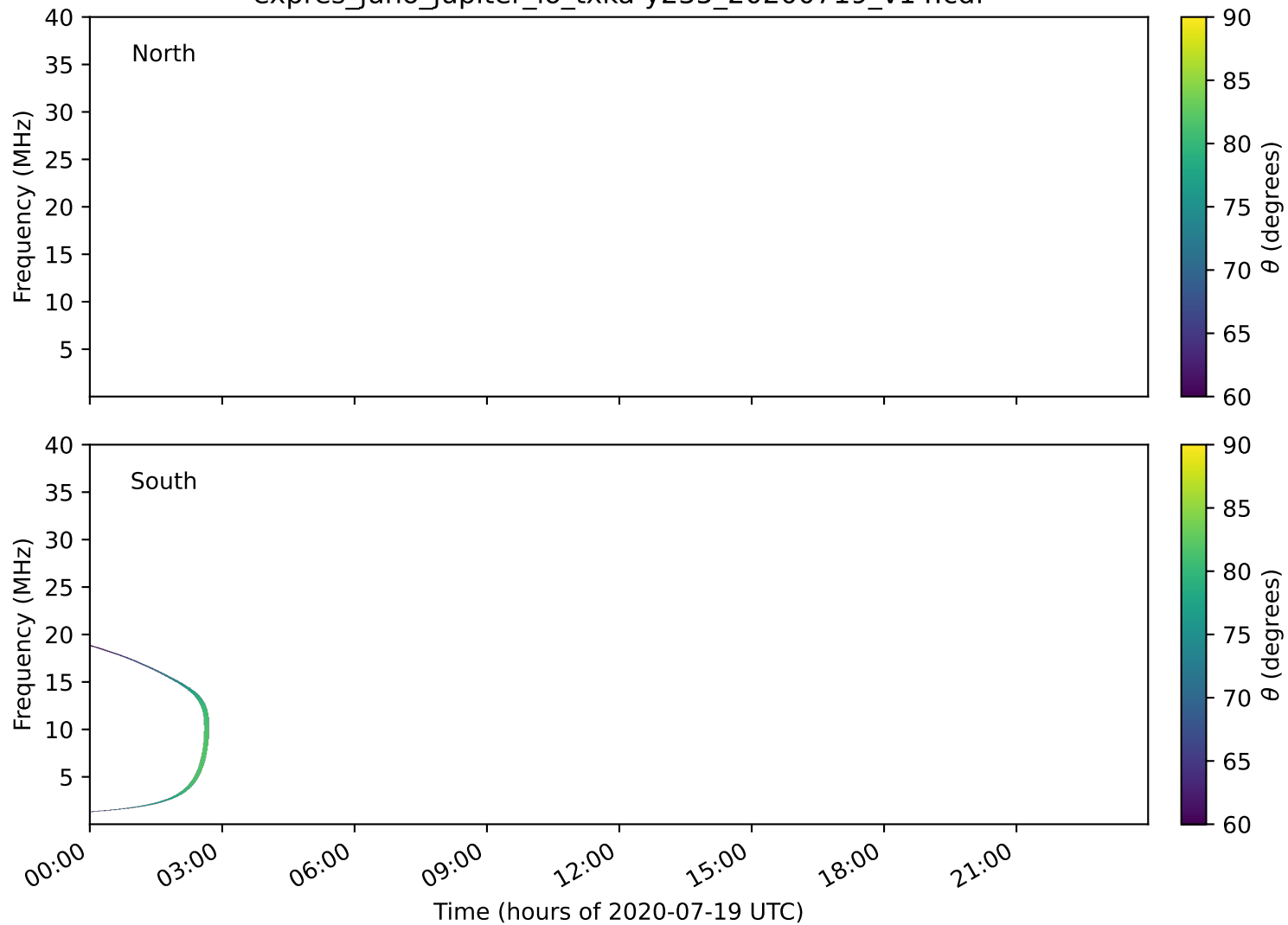
expres_juno_jupiter_io_txka-y235_20200719_v14.cdf
