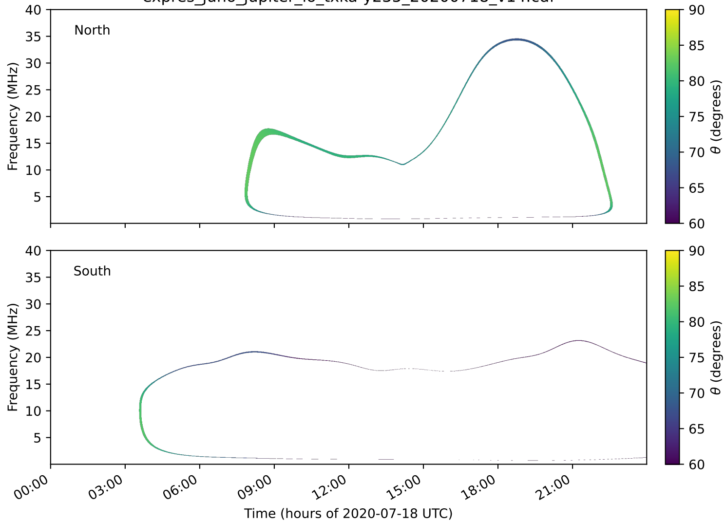
expres_juno_jupiter_io_txka-y235_20200718_v14.cdf
