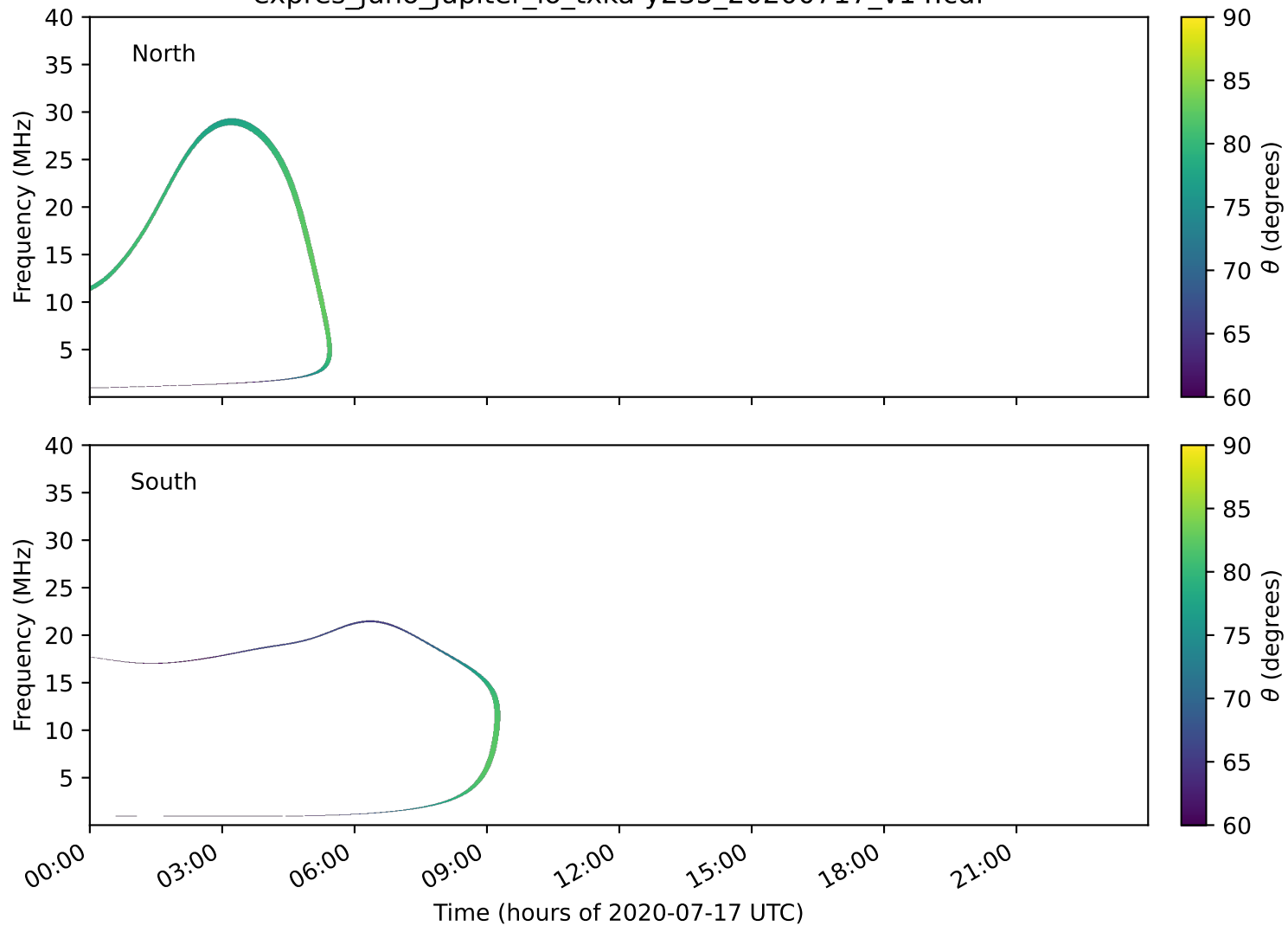
expres_juno_jupiter_io_txka-y235_20200717_v14.cdf
