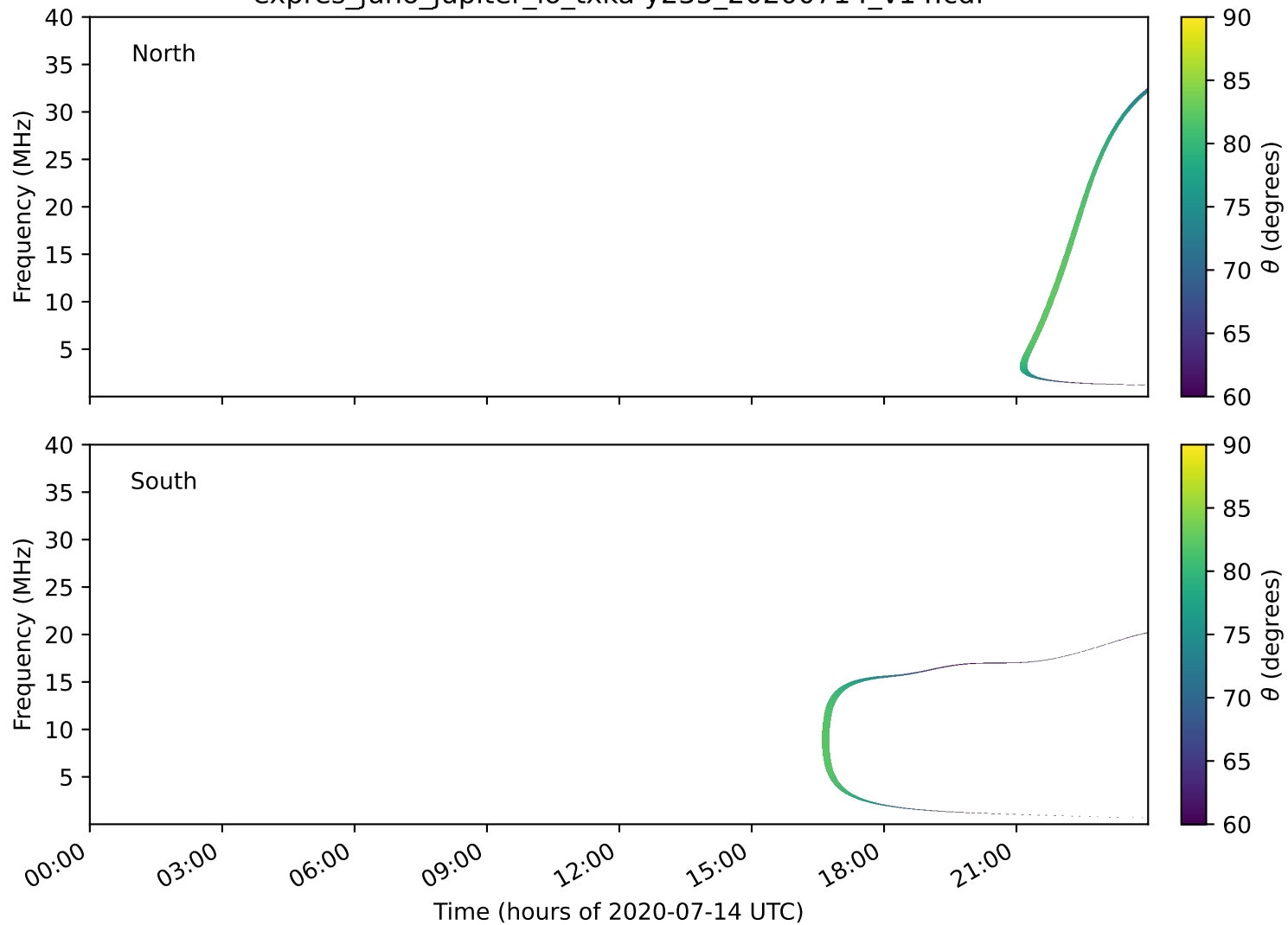
expres_juno_jupiter_io_txka-y235_20200714_v14.cdf
