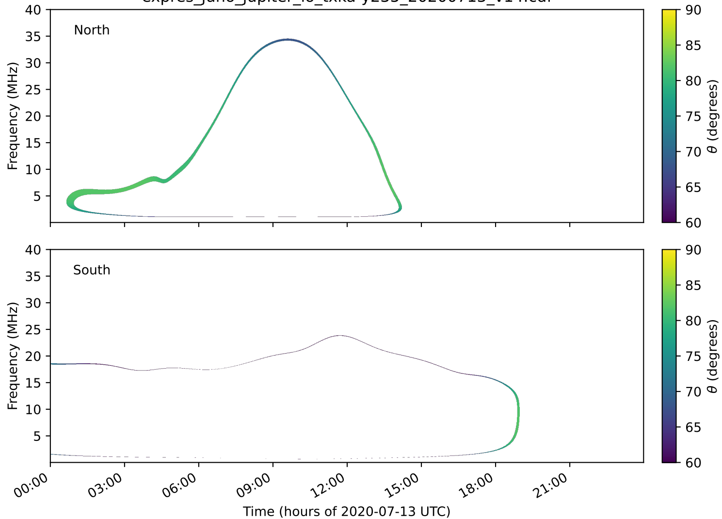
expres_juno_jupiter_io_txka-y235_20200713_v14.cdf
