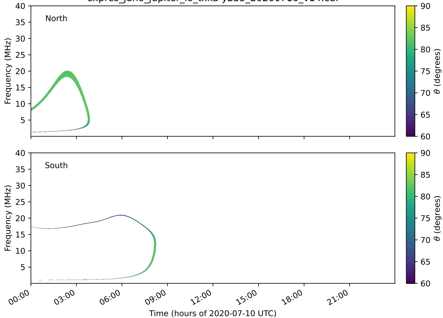
expres_juno_jupiter_io_txka-y235_20200710_v14.cdf
