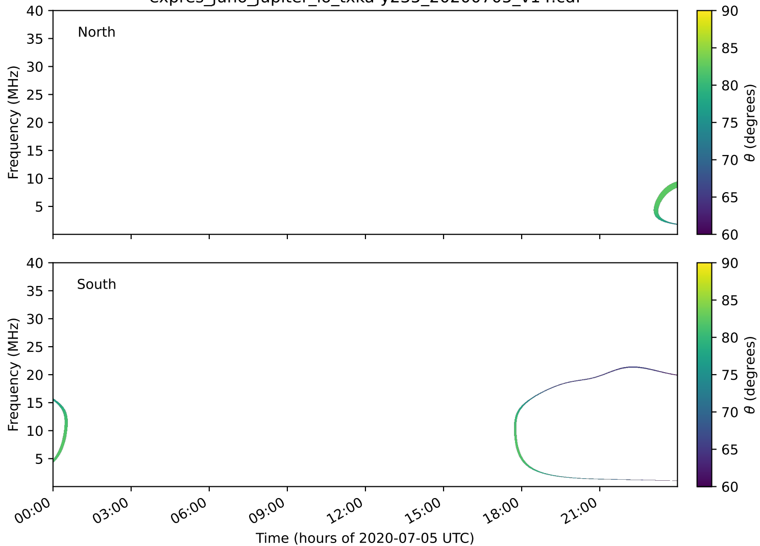
expres_juno_jupiter_io_txka-y235_20200705_v14.cdf
