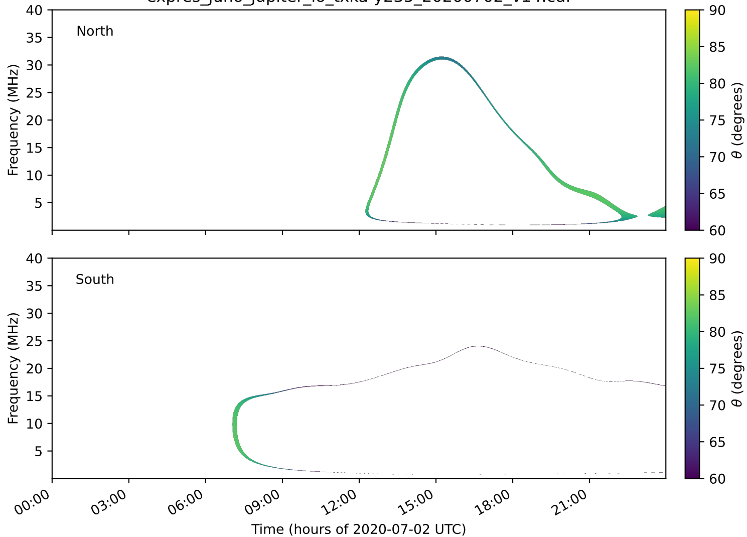
expres_juno_jupiter_io_txka-y235_20200702_v14.cdf
