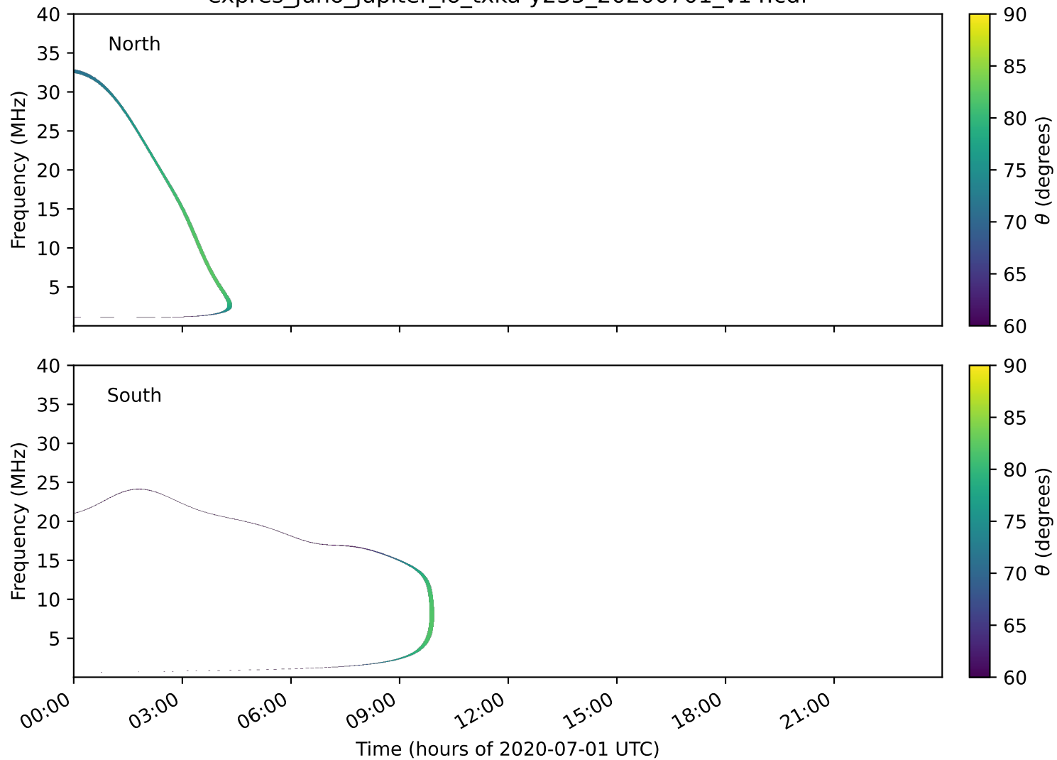
expres_juno_jupiter_io_txka-y235_20200701_v14.cdf
