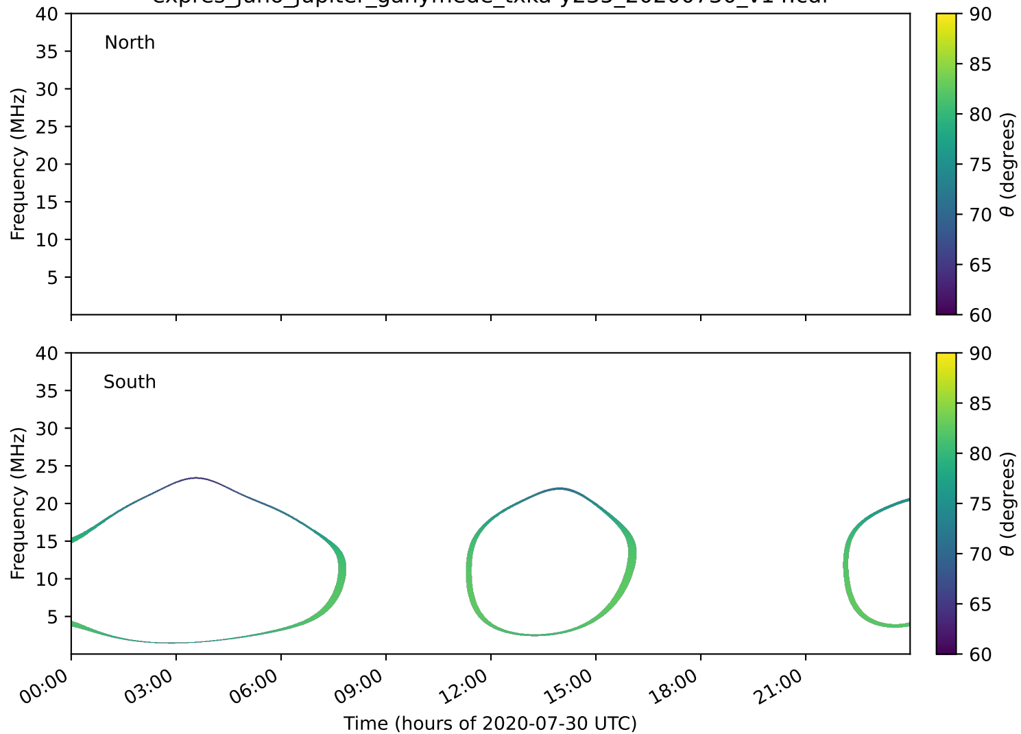
expres_juno_jupiter_ganymede_txka-y235_20200730_v14.cdf
