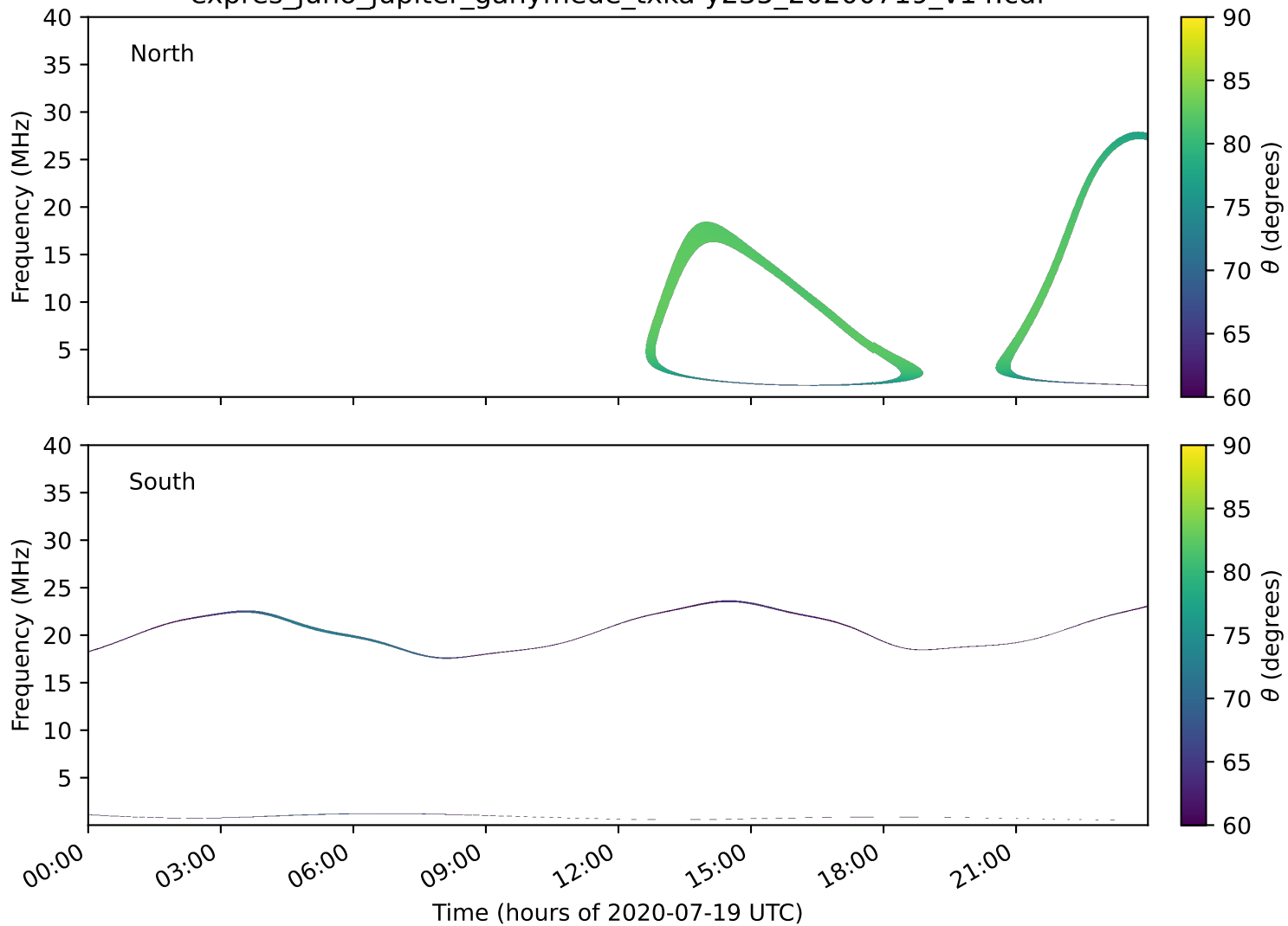
expres_juno_jupiter_ganymede_txka-y235_20200719_v14.cdf
